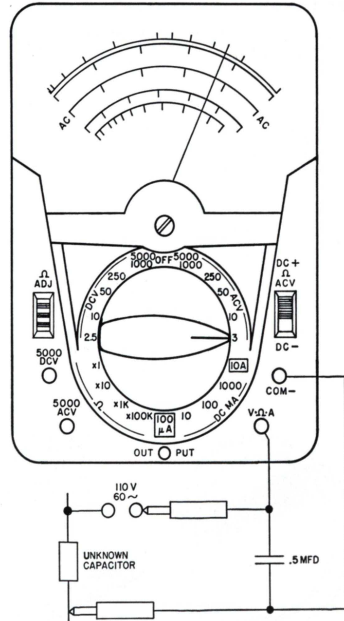
Figure 6—Measuring Capacity
