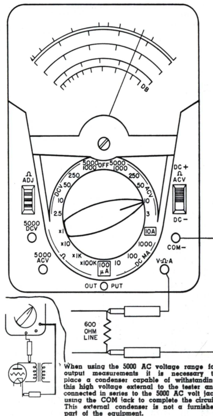
Figure 5—Measuring Output Volts (DB)
