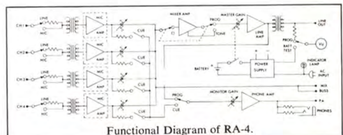
Functional Diagram of RA-4.
