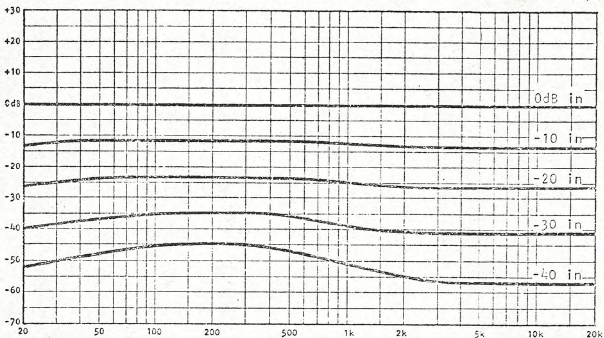
Fig. 3-5, WIDEBAND NOISE
