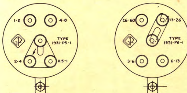
Figure 1. Range-selecting terminals for input tuning coils.
