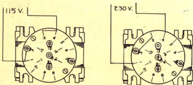
Figure 2. Power transformer connections for 115 volts and 230 volts.
