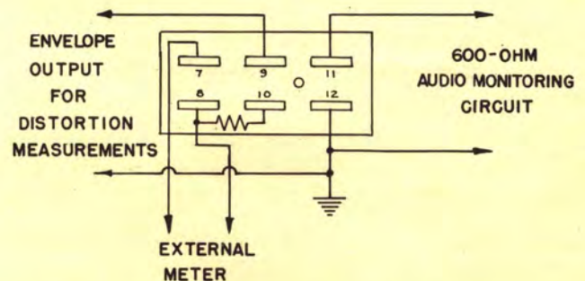
Figure 3. Rear connections.
