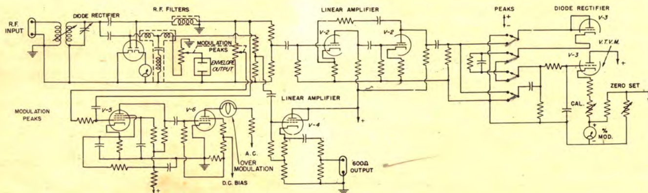
Figure 4. Elementary schematic circuit diagram.
