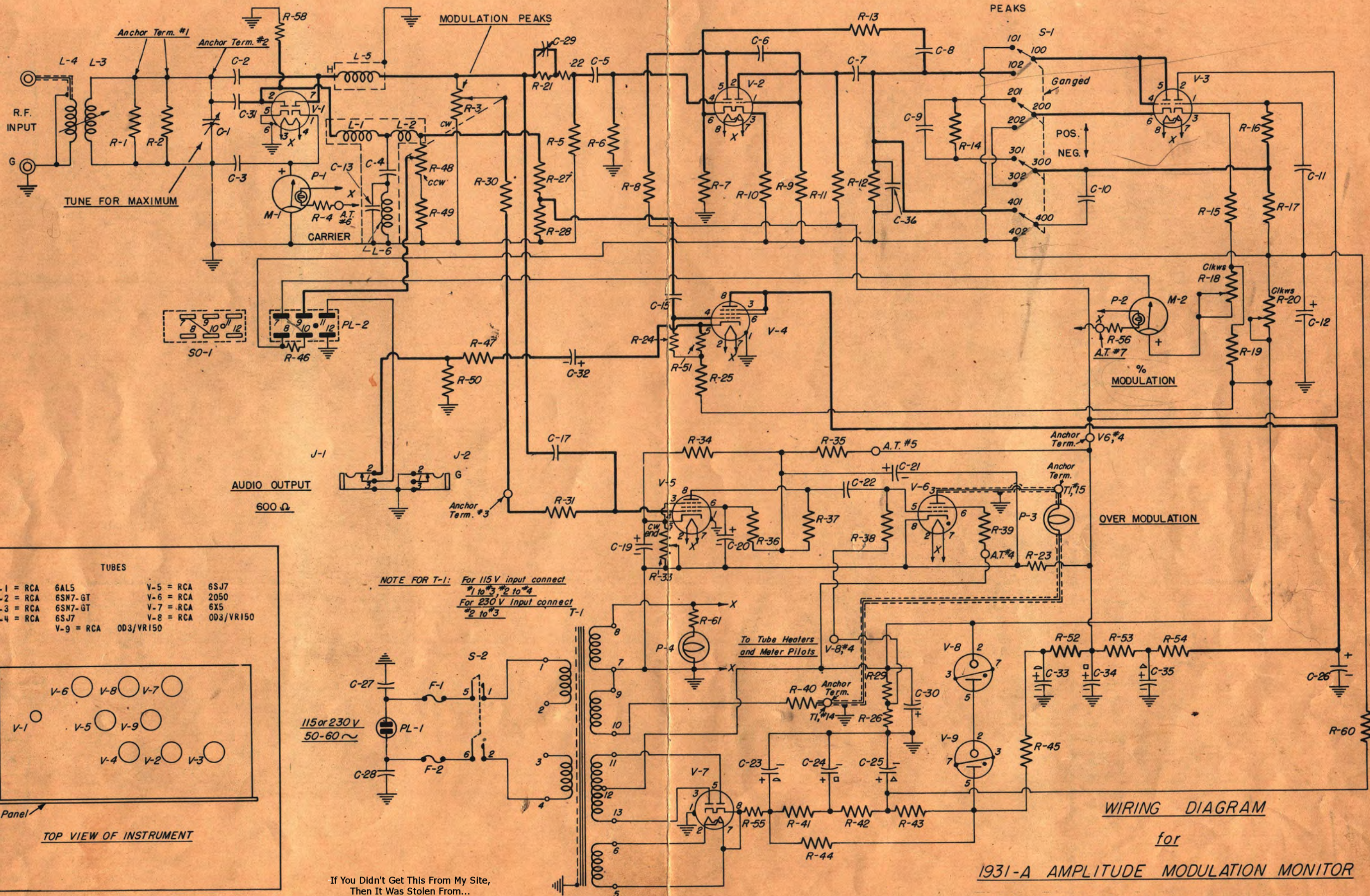
Figure 5. Complete wiring diagram and tube layout.
