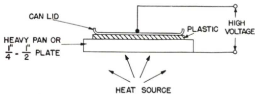
Fig. 3. Arrangement for charging the electret
