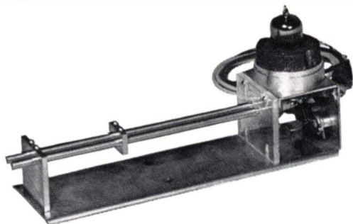
Fig. 8. Experimental test arrangement for Z-2061 magnetron
