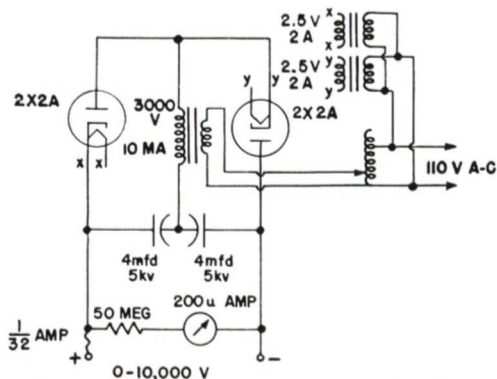
Fig. 5. High voltage power supply suitable for making electret
