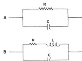
Fig. 12. Equivalent circuits
