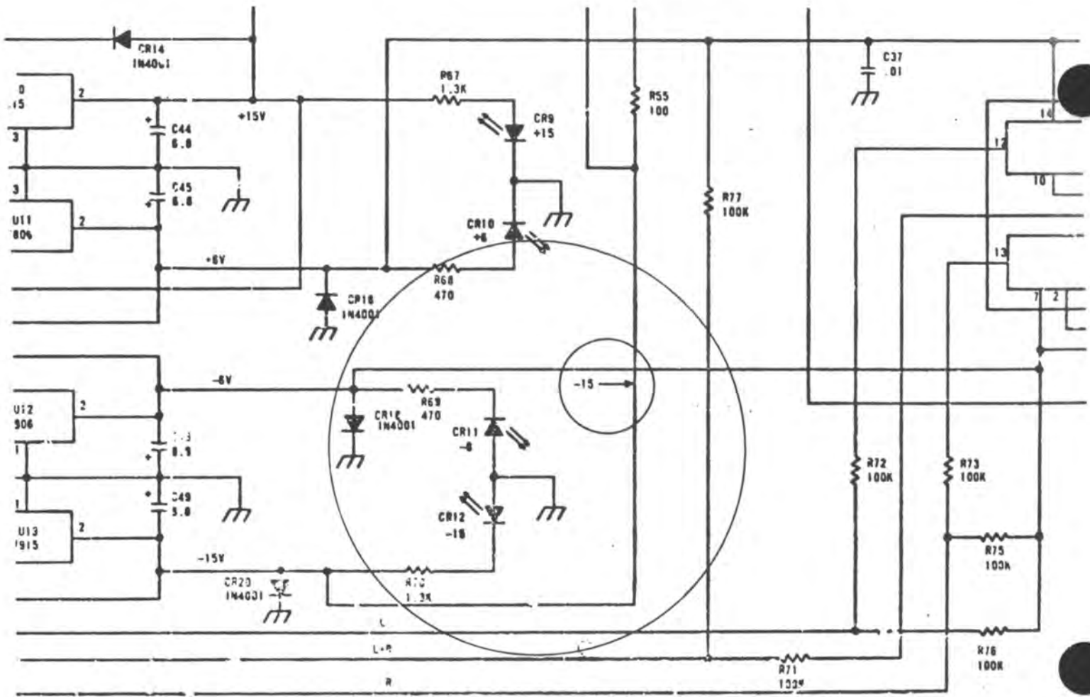
Location of Arrow Insertion on schematic 852 8408 001 to update to Rev. E.
