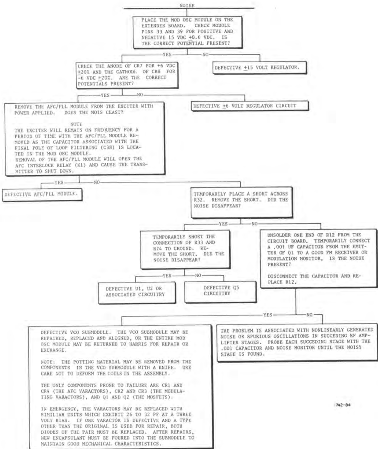
Figure 5-6. Noise
