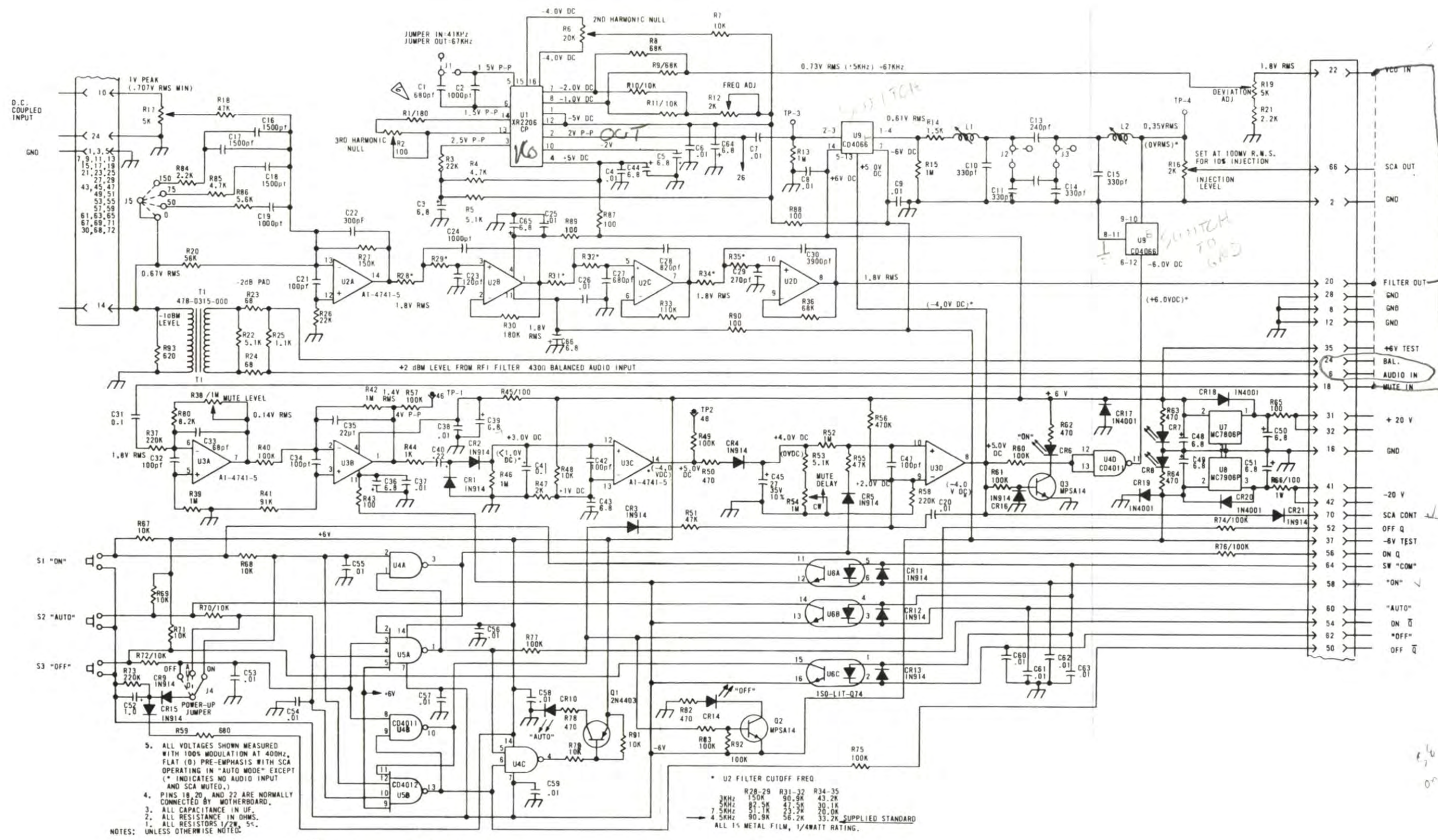
FIGURE 5-3. SCA MODULE SCHEMATIC 843 1696 001
