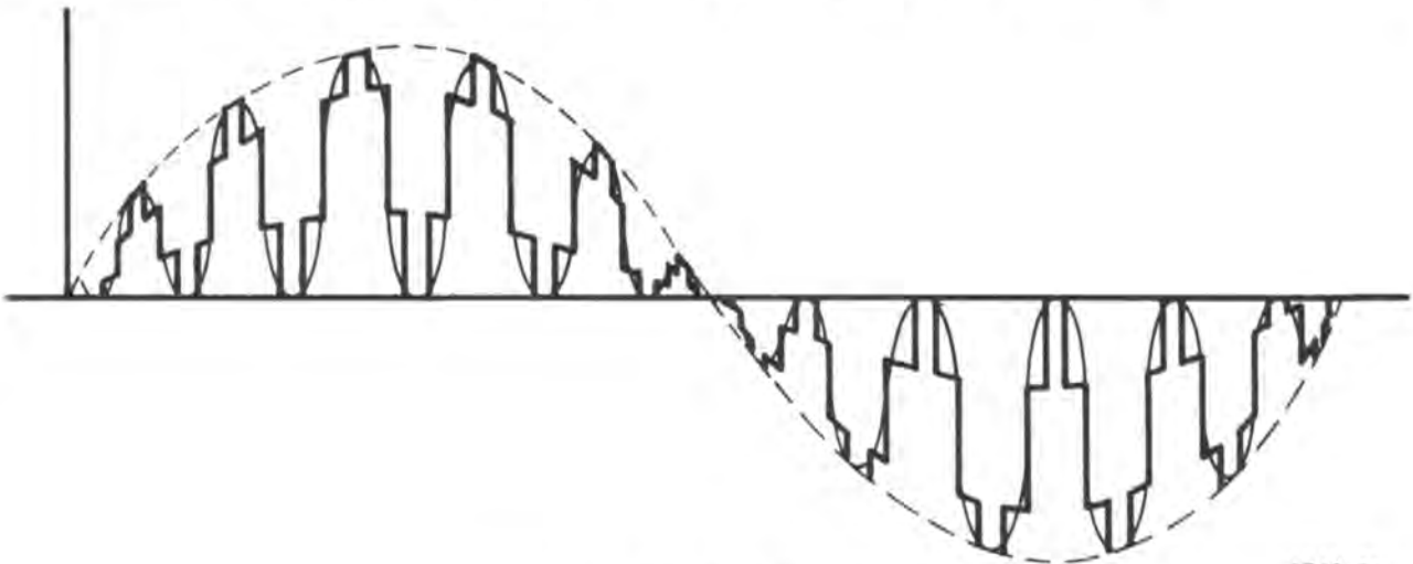
Figure 4-2. DSM Waveform
