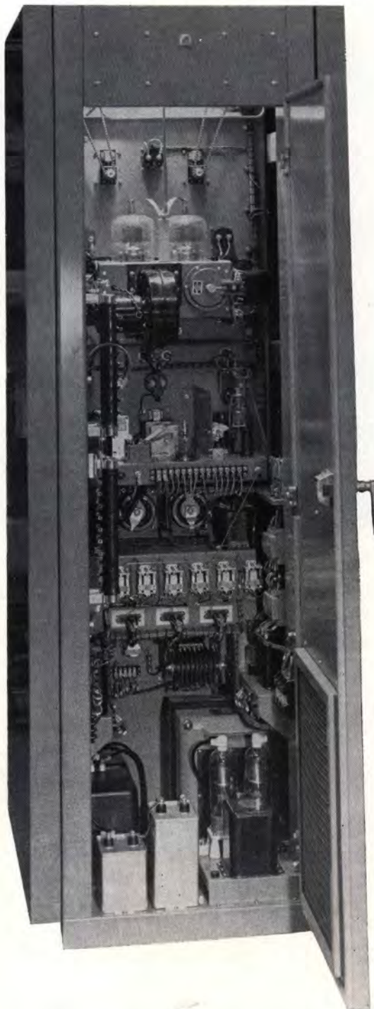
A glance inside the CMP-1 transmitter instills confidence of dependability. You will note the husky components, neat workmanship and symmetrical arrangement of components for proper electrical design.
