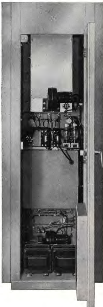
REAR—FMR-250 Transmitter
