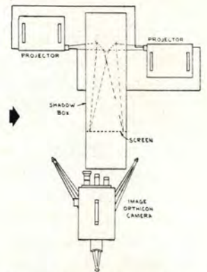
Above illustrates dual projectors into a single Image Orthicon camera by use of a simple light-tight shadow box 76" long. This provides a picture 11"x14" in size. Screen is set back in shadow box to prevent front lighting.
