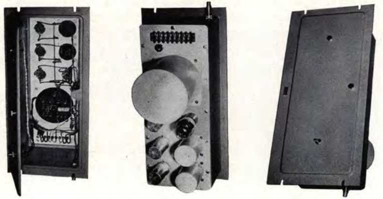
Above are front, internal and rear views of the rack mount power supply part of the SA-40 equipment.
