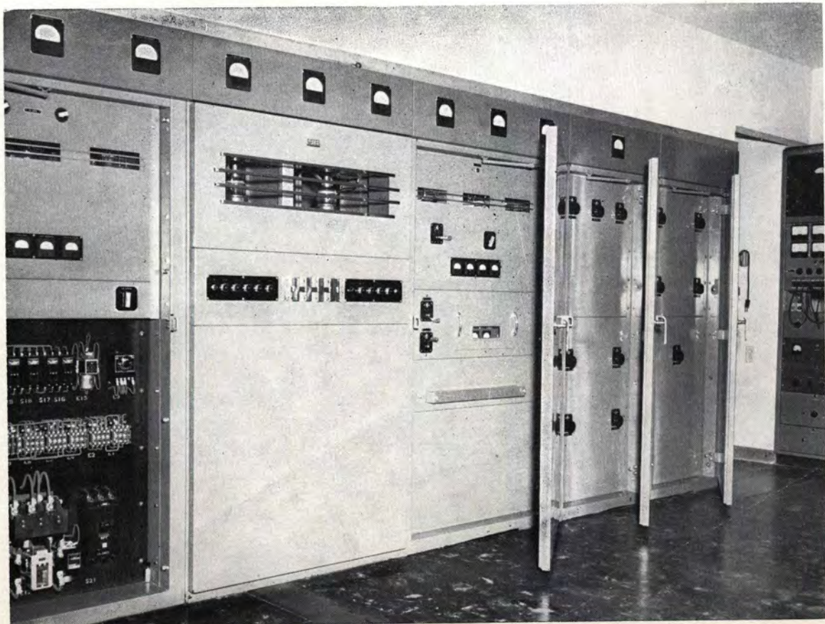
Below—Gates BC-5B 5000 watt equipment with five tower phasing equipment in matching cabinet at WENE, Endicott, N. Y.
