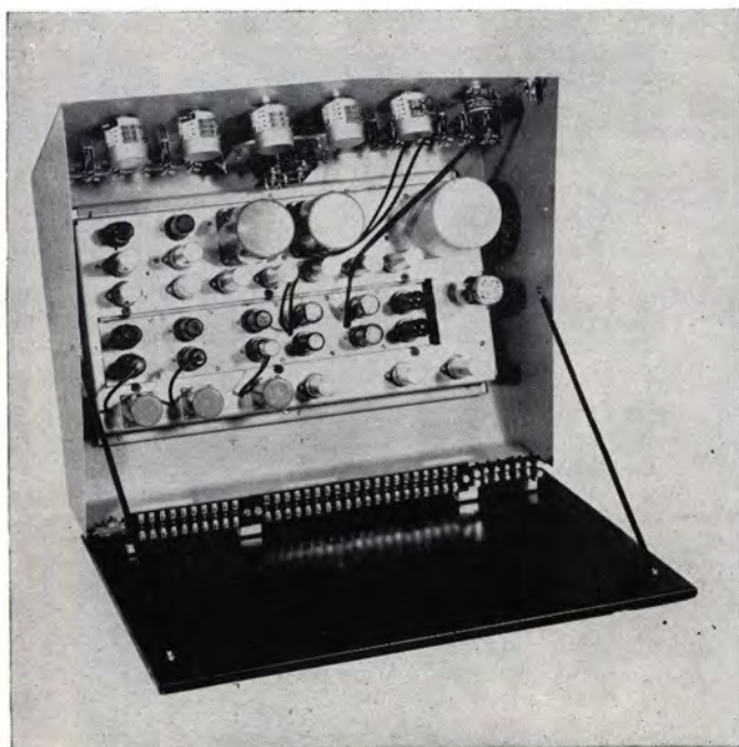
The above illustrates the tilt-back arrangement of the Studioette cabinet for reaching tubes, attenuators, and terminal connections instantly. For reaching under-chassis parts, the top of the cabinet is removable, making complete instantaneous 100% accessibility possible.
