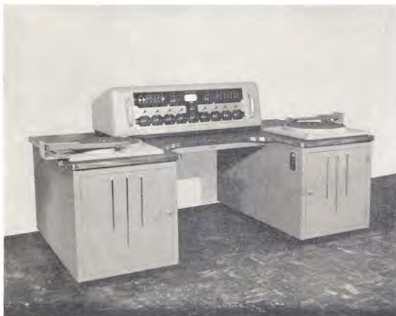
Illustrated to the left is the SA-40 Console mounted on the popular Gates CB-4 horseshoe desk with CB-11 transcription turntables on each wing of the horseshoe. The CB-4 desk offers commanding appearance and will be found in leading broadcasting stations throughout the country. See page 35.
