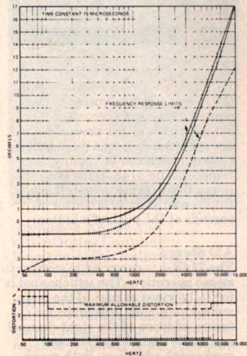
Stereo: Left Channel Response and THD
