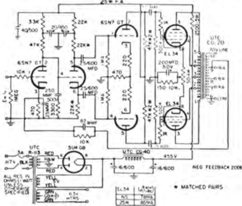
CIRCUIT PROVIDING 25 WATTS, ± 1 db 40 Hz to 10 kHz . . . At 1 watt, ± 1 db 20 Hz to 20 kHz.
