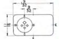
TMN-4 thru TMN-1.7 1 1/4" x 1 1/2" x 2" Weight ... 3.5 oz.
