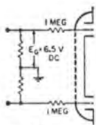
FIG #2 GRID CIRCUIT MODIFICATION FOR DC INPUT
