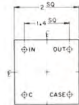
FP-A \frac{1}{2} " HIGH; WT: 2.5 OZ
