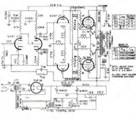
CIRCUIT PROVIDING 35 WATTS, ± 1 db from 15 Hz to 30 kHz . . . At 1 watt, ± 1 db 7 Hz to 100 kHz.
