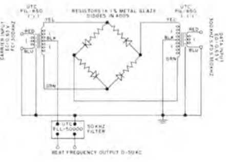
BALANCED MODULATOR—BEAT FREQUENCY MIXER
