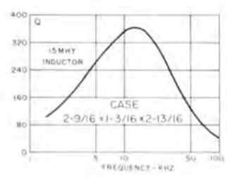
Type MQV, 15 millihenries temperature stable inductor. High Q in the 2 kHz to 50 kHz frequency range. MIL-T-27C. Wt. 14 oz.
