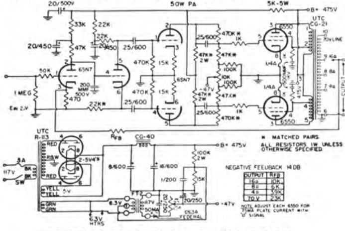
CIRCUIT PROVIDING 50 WATTS, ± 1 db 40 Hz to 10 kHz . . . At 1 watt, ± 1 db 20 Hz to 20 kHz.
