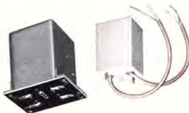
Special chopper type transformers with terminals or shielded leads; multiple high permeability magnetic shields; electrostatic shielding for voltage isolation of 2 x 10 6 .
