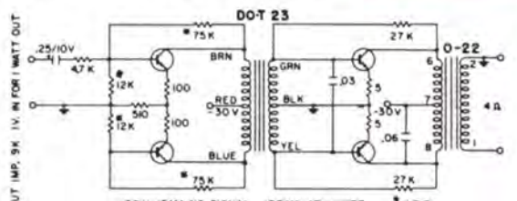
Circuit providing 1 watt, frequency range 200 Hz to 20 kHz
