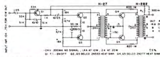
Circuit providing 20 watts, frequency range 50 Hz to 20 kHz
