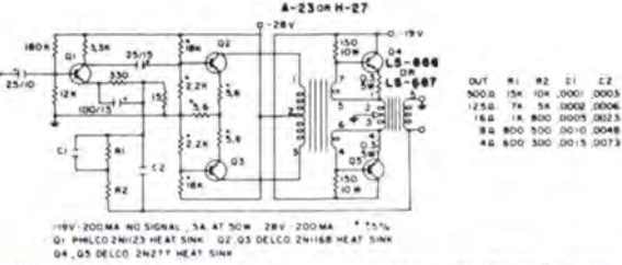
Circuit providing 50 watts, frequency range 20 Hz to 20 kHz
