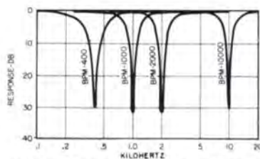
TYPICAL BAND REJECT RESPONSES
