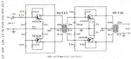
Circuit providing 350 mw, frequency range 900 Hz to 160 kHz
