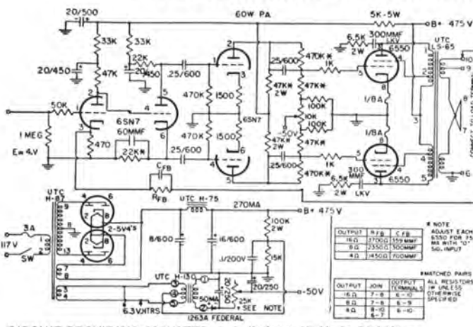
CIRCUIT PROVIDING 60 WATTS, ± 1 db from 15 Hz to 30 kHz . . . At 1 watt, ± 1 db 3 Hz to 80 kHz.
