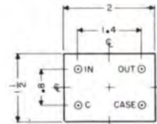
FP-C \frac{1}{2} " HIGH; WT: 2.2 OZ
