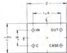
FP-B \frac{3}{8} " HIGH; WT: 2 OZ
