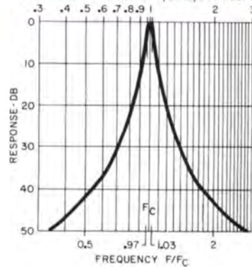
TYPICAL NORMALIZED BMI, BML, BTI RESPONSE
