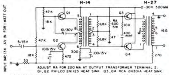
Circuit providing 1 watt, frequency range 40 Hz to 20 kHz
