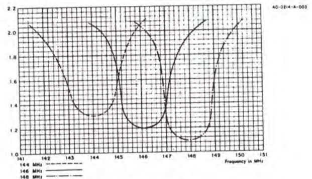
Figure 3A VSWR for Horizontal Polarization Only
