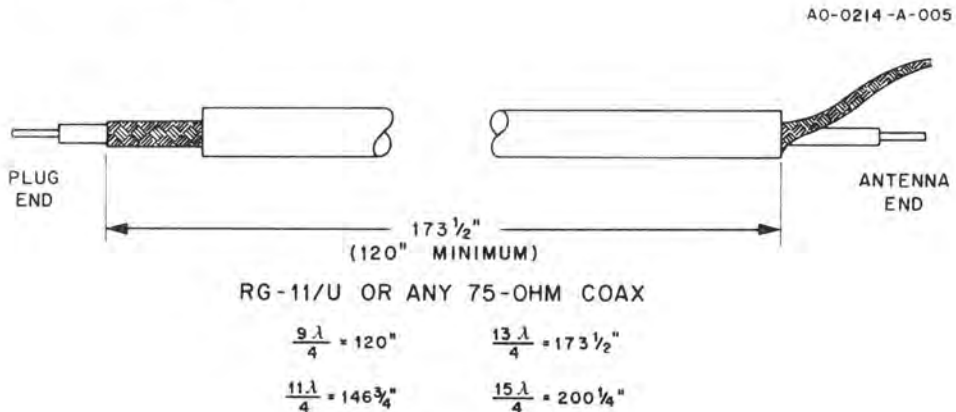
Figure 5 Coaxial Cable Length for Phasing
