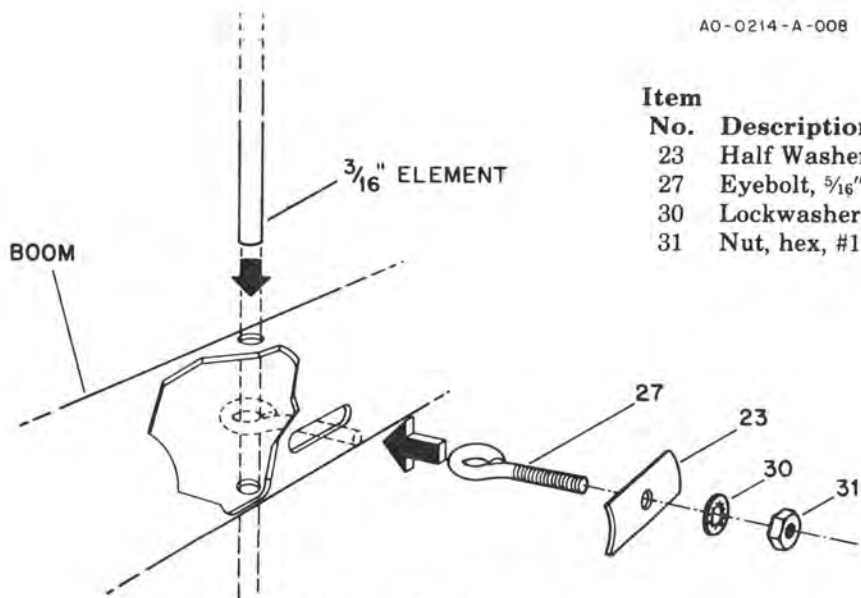
Figure 6 – Detail A Element Assembly
