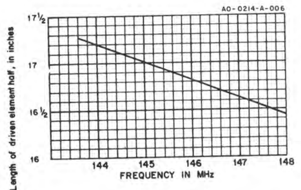
Figure 3B Driven Element Cutting Chart
