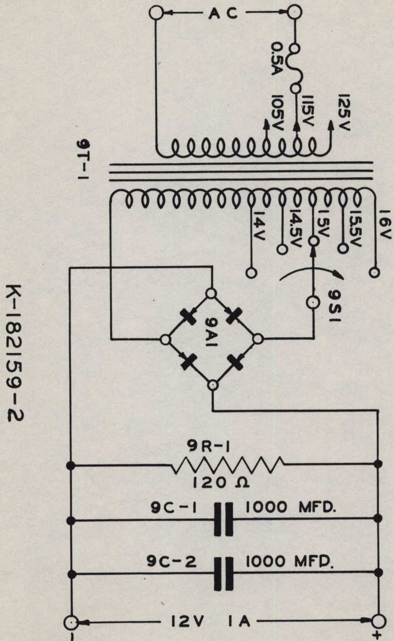
Figure 7—Relay Power Supply, Schematic (K-182159)
