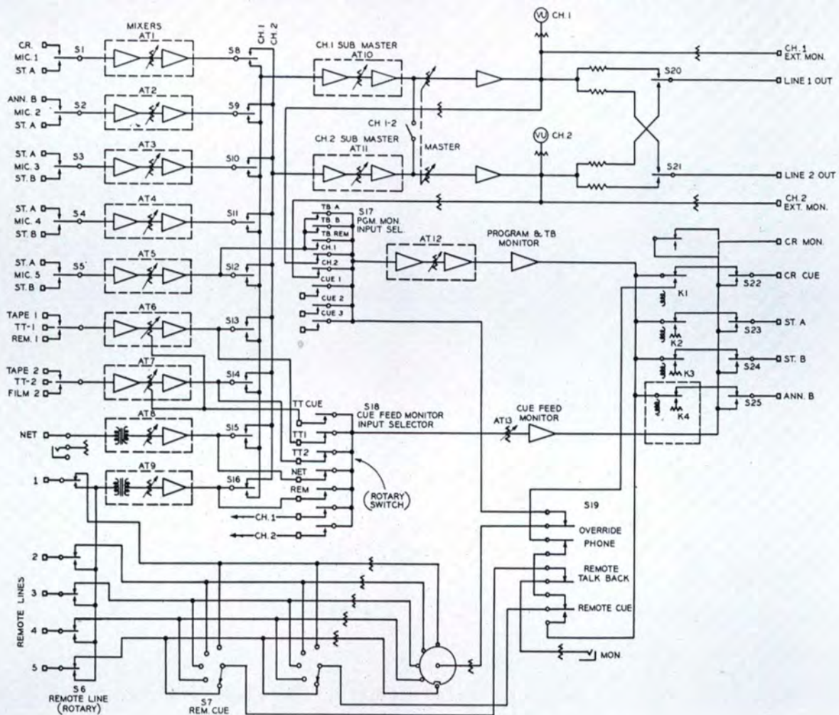
Simplified block diagram of the BC-6A Dual-Channel Audio Console.
