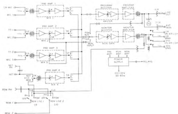
Simplified block diagram of BC-5A Consolette.
