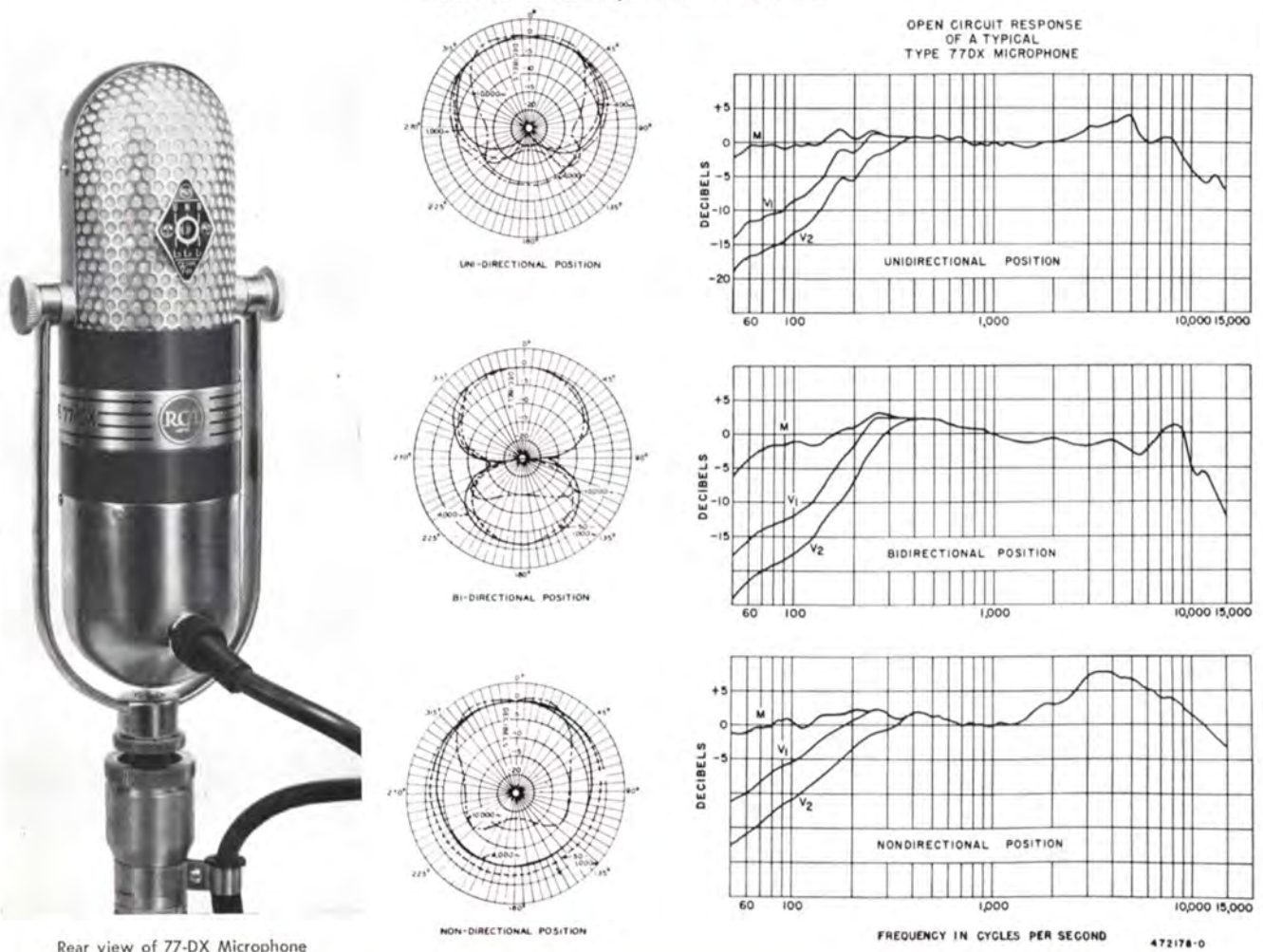
Rear view of 77-DX Microphone
