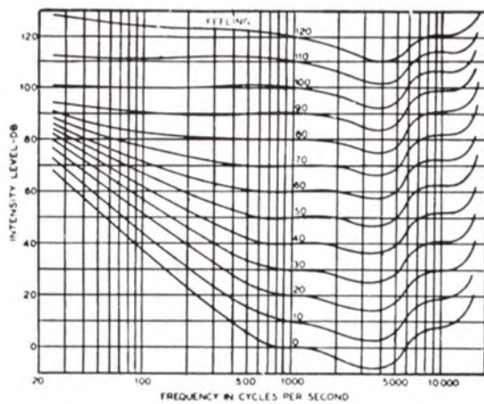
Loudness level contours.
