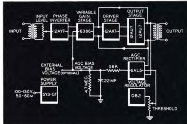
Simplified Block Diagram of BA-25A AGC Program Amplifier
