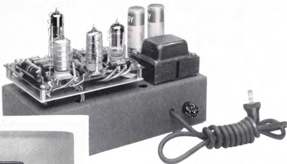
Rear view of BN-5A Amplifier with cover removed showing components mounted on removable etched wiring board and self-contained power supply.
