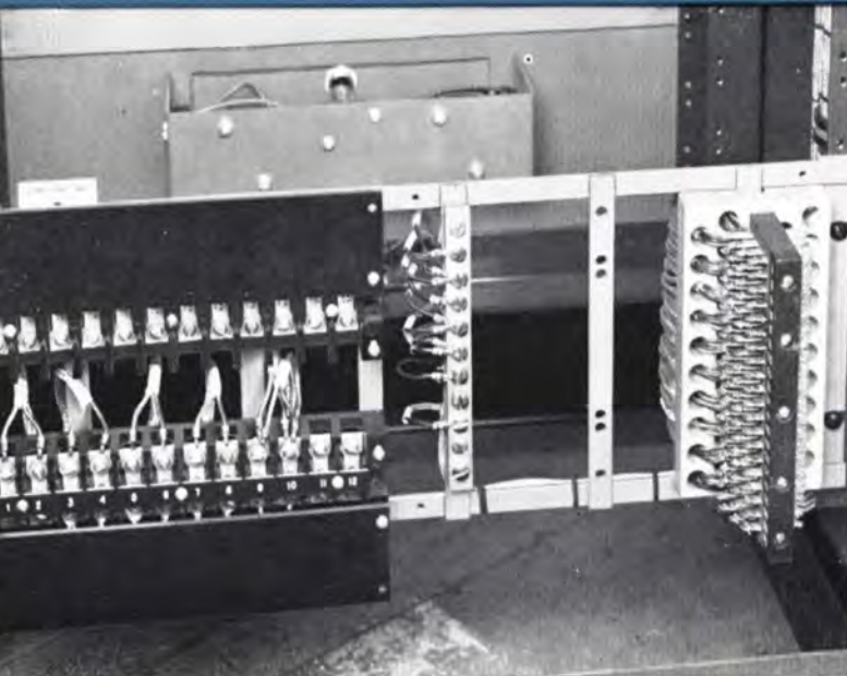
Fig. 1. Photo of terminals at bottom of rack. Power terminals are at left, ground buss in center and audio terminals at right.
