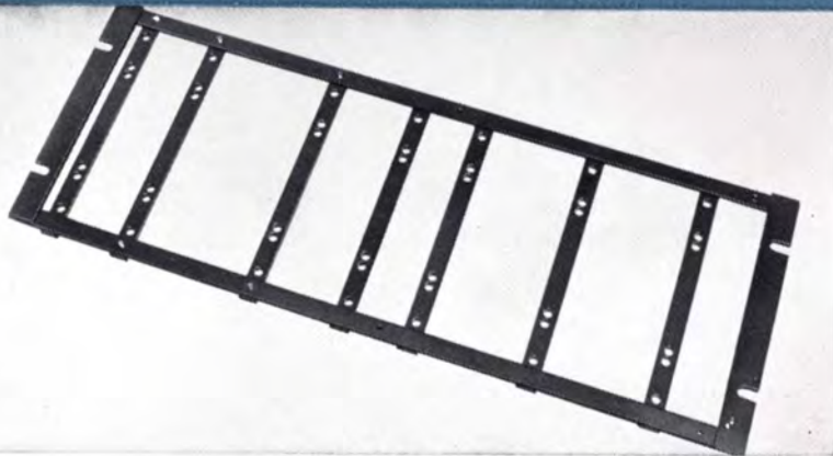
Terminal Block Mounting Bracket MI-4570-A.
