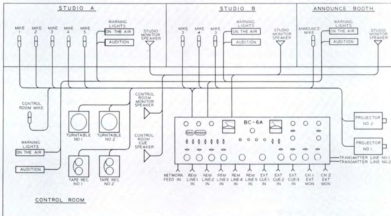
Simplified Facilities Diagram for the new RCA Type BC-6A Split-Mixer, Dual Channel Audio Consolette.
