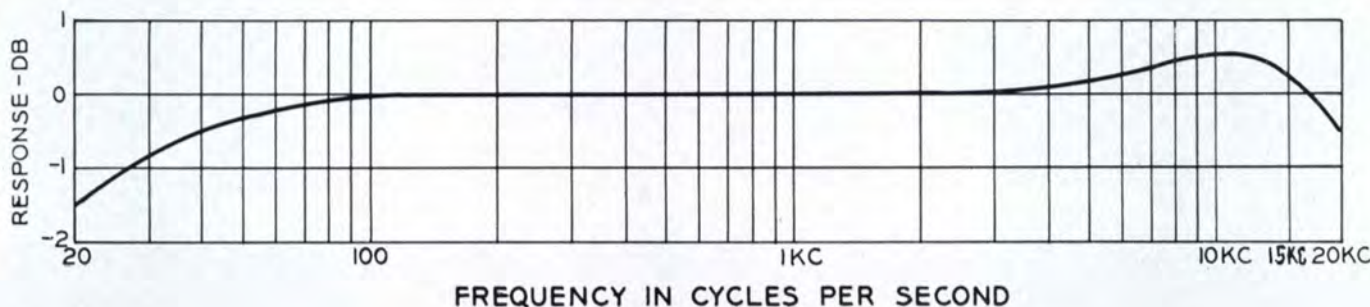
FREQUENCY RESPONSE MI-11247 MONITOR AMPLIFIER TYPE - BA-24A
