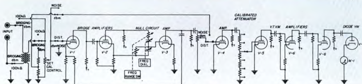
Elementary schematic circuit diagram of the WM-71A Distortion and Noise Meter.
