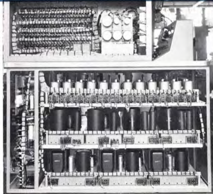
Fig. 2. View of wiring in a control desk. A-c circuits are below the shelves, and audio above.
