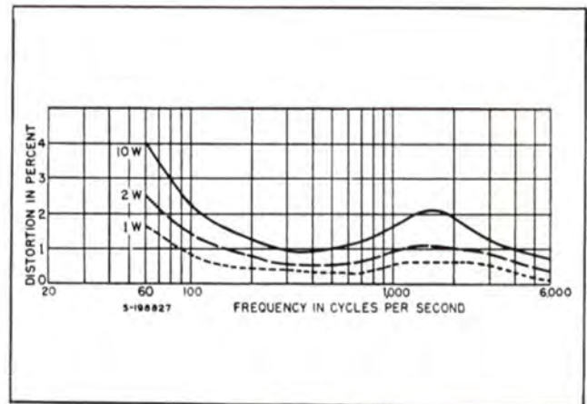
Harmonic Distortion of LC-1A Speaker.
