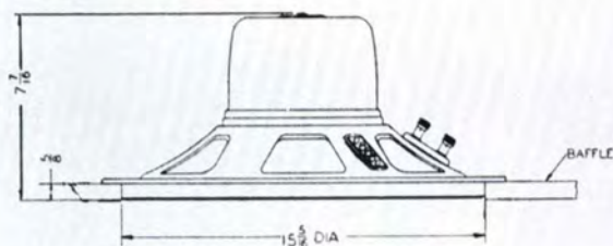
Dimensions of LC-1A Speaker
