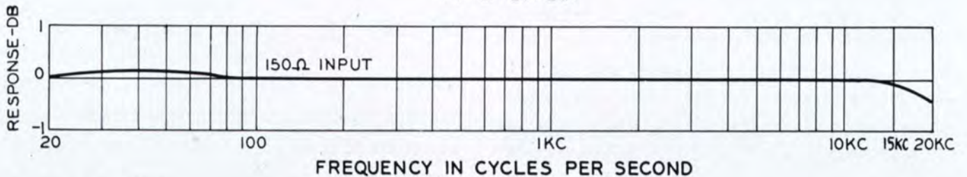
TYPICAL FREQUENCY RESPONSE MI-11244 PRE-AMPLIFIER TYPE-BA-21A
