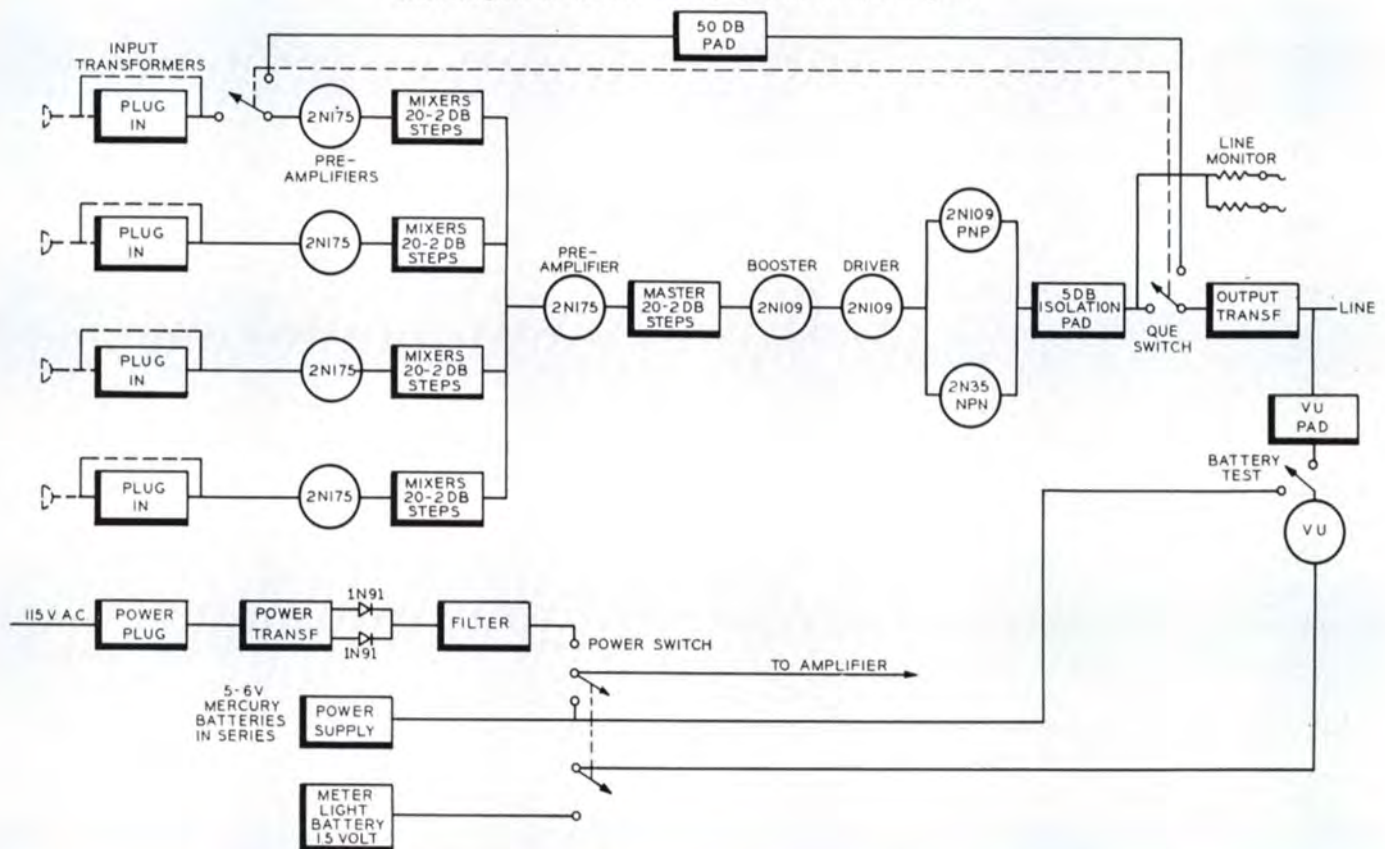
Block Diagram of BN-6A Transistor Portable Remote Amplifier
