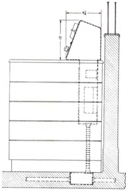
This cross-section view shows how the console at right was designed to permit some components to be mounted below the desk top. This results in small turret size and provides maximum visibility into the studio.
