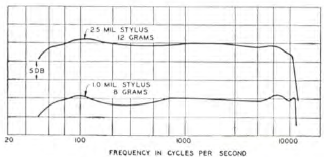
Typical response of Pickup, Tone Arm and Filter.
