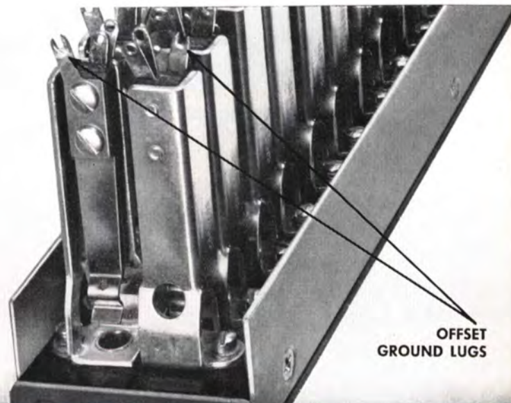
Photo below shows Convenient Offset Ground Lugs
