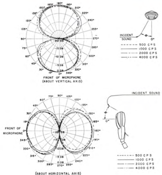
Directional Characteristics of the SK-35 and SK-46 Velocity Microphones.
