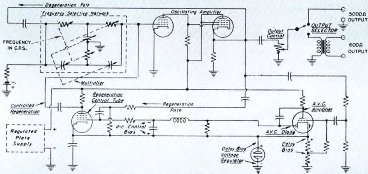
Elementary schematic circuit diagram of the WA-28A Low Distortion Oscillator.
