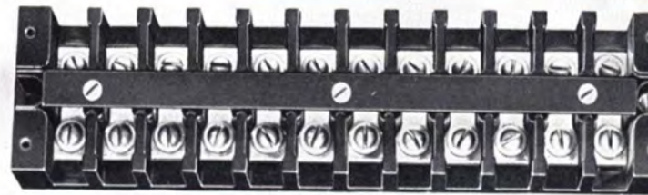
Power Terminal Block MI-4568 with cover removed.
