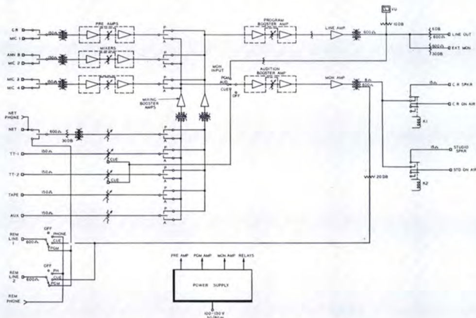
Simplified block diagram of the BC-3B Standard Console.
