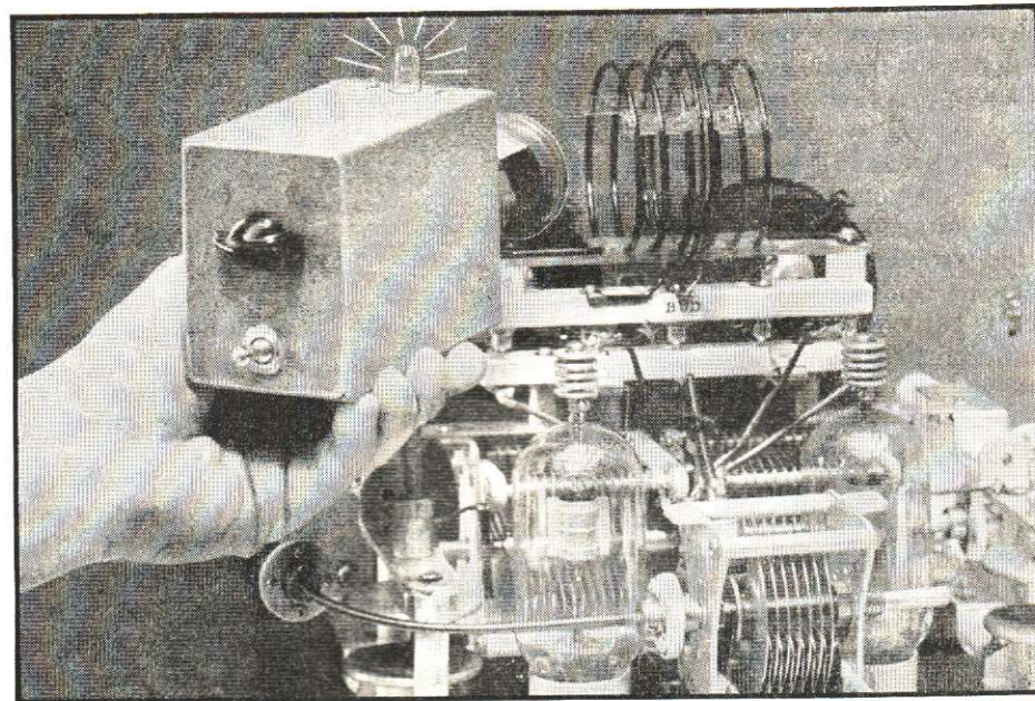
There are plenty of coils in this interesting view of the r.f. section of a short-wave transmitter. The transmitter coils, without cores and with plastic spacer bars instead of forms, are prominent on top of the assembly. The box with a coil projecting from its back is a wavemeter, used to determine the approximate frequency at which the transmitter is operating. The bulb on top of the box lights up when the transmitter is properly adjusted.
