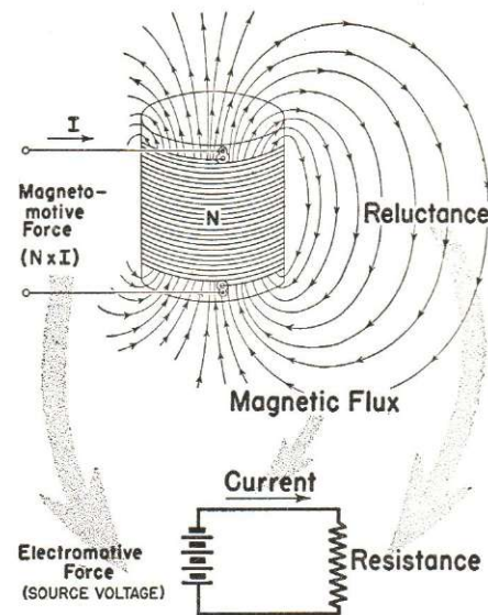
FIG. 4. Similarity between magnetic and electric circuits. The total reluctance is here the reluctance of the air through which the magnetic flux loops flow. Lines of force go out of the ends of the coil in all directions, but only a few of the lines can be shown in a diagram of this nature.
