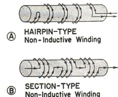
FIG. 21. Two ways of winding wire-wound resistors so they have practically no inductive characteristics. Arrows indicate directions of electron flow.
