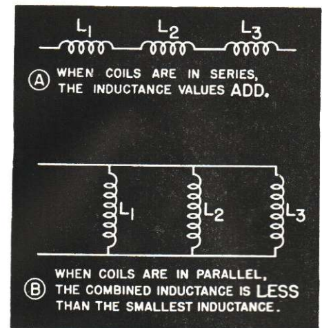
FIG. 18. Coils combine exactly like resistors.
