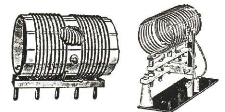
Air-core transformers for short-wave transmitters. The amount of coupling between the two coils is varied in the left-hand unit by rotating a small inner coil, and in the right-hand unit by moving a link (one or two-turn coil) between the two coils.
