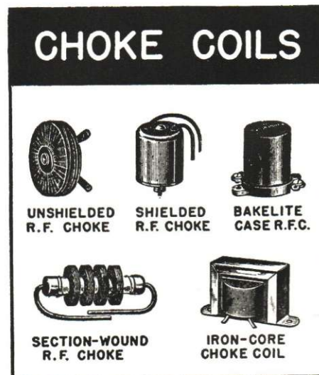
Examples of choke coils you will encounter in radio receivers and transmitters. Single coils by themselves are called choke coils by radio men, and are used individually in radio circuits to offer opposition to alternating current without appreciably hindering the flow of direct current. Basket-weave windings (like that of the unshielded r.f. choke) and criss-cross windings give low distributed capacity (explained later), thereby improving the effectiveness of the coil at high radio frequencies.
