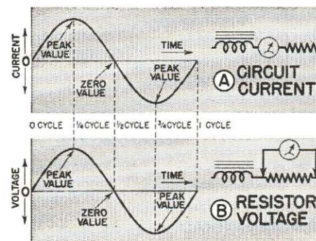
FIG. 23. These two curves show that voltage and current values for a resistor reach corresponding values at exactly the same instant of time. This means that voltage and current for a resistor are IN PHASE with each other.
