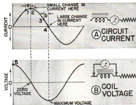
FIG. 24. The basic fact that a coil voltage is OUT OF PHASE with the coil current is shown by these two curves.
