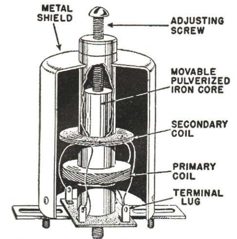
R.F. transformer with adjustable pulverized iron core. Tightening the adjusting screw raises the core out of the primary coil, thereby reducing the amount of coupling between the two coils.
