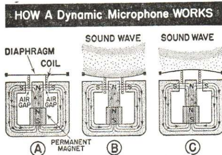
FIG. 15. Simplified cross-section views of a dynamic microphone.
