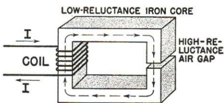
FIG. 5. The flux produced by this coil travels along a magnetic circuit consisting of an iron core and a short air gap. The total reluctance is but slightly higher than the air gap reluctance.
