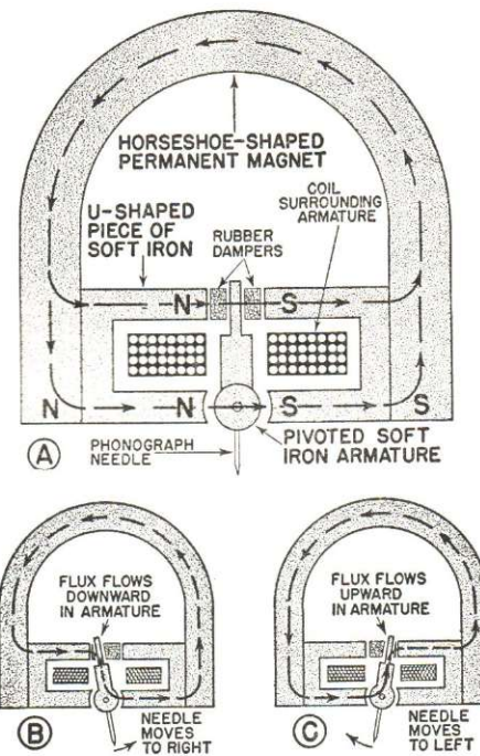
FIG. 16. Cross-section views illustrating the basic operating principles of a magnetic phono pick-up.
