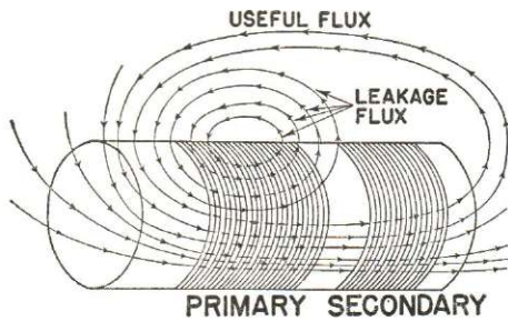
FIG. 19. Leakage flux. In the average coil, the leakage flux is only a small proportion of the total useful flux.
