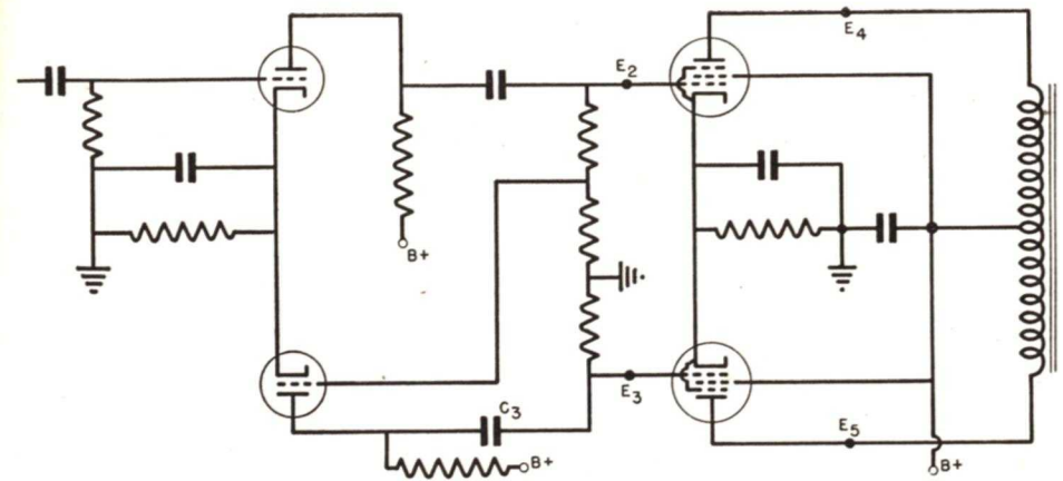
FIG. 3. Typical output stage of a p.a. amplifier.
