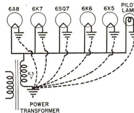
FIG. 23. Filament circuit, with dotted lines indicating the connections that are completed through the chassis of the receiver. All tube filaments and the pilot lamp require 6.3 volts, and the transformer secondary provides this voltage.
