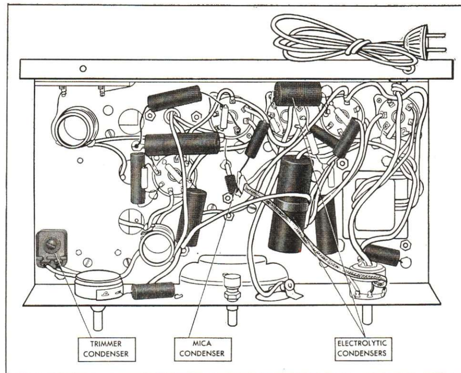
FIG. 17. This shows the condensers underneath the chassis of our superhet receiver. The condensers not marked are paper condensers.
