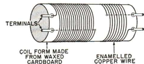
FIG. 20. Construction of an r.f. coil.
