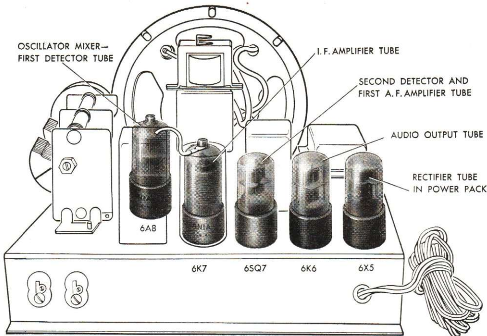
FIG. 9. This is the back of our superheterodyne receiver chassis showing the tubes.
