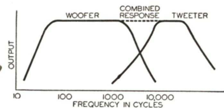
FIG. 27. Response curves for a high-fidelity, two-loudspeaker arrangement.
