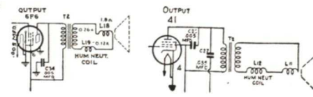
FIG. 26. Schematic circuit diagrams of radio receivers usually indicate, in a manner similar to that shown above, whether a hum-neutralizing (hum-bucking) coil is used in the loudspeaker.
