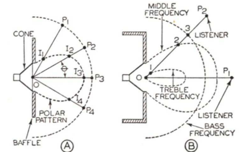
FIG. 17. Polar sound radiation patterns for cone loudspeakers.
