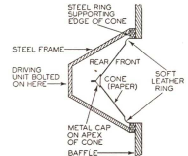
FIG. 1. Cross-section view of a cone loudspeaker and its supporting structure, as mounted on a wood baffle. Driving unit is not shown.
