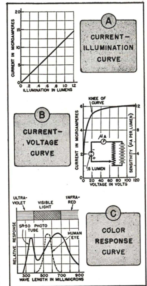
FIG. 7. Typical characteristic curves for vacuum type photoemissive cells. (These curves are for the Westinghouse SR-50 photocell.)
