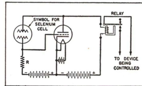
FIG. 13. Notice the symbol used to represent the selenium cell in this basic circuit.
