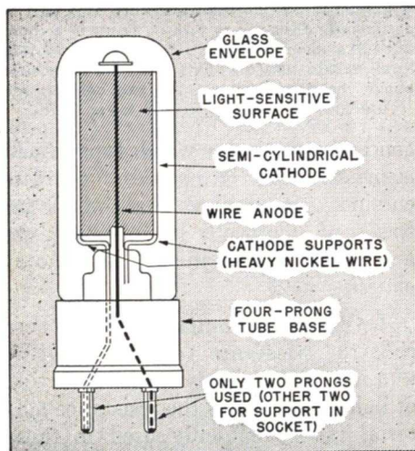
FIG. 4. The connections and parts of a photoemissive cell.
