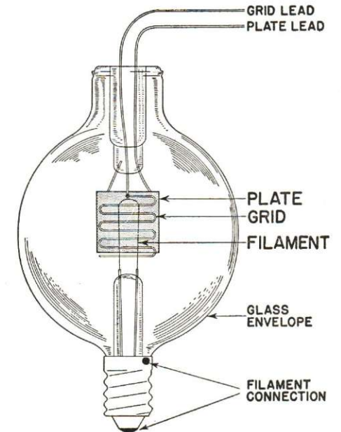
FIG. 13. DeForest "audion" radio tube, sketched from a tube in the N.R.I. collection of history-making tubes. If you ever visit N.R.I., be sure to look for this audion tube in the display rack on the third floor.
