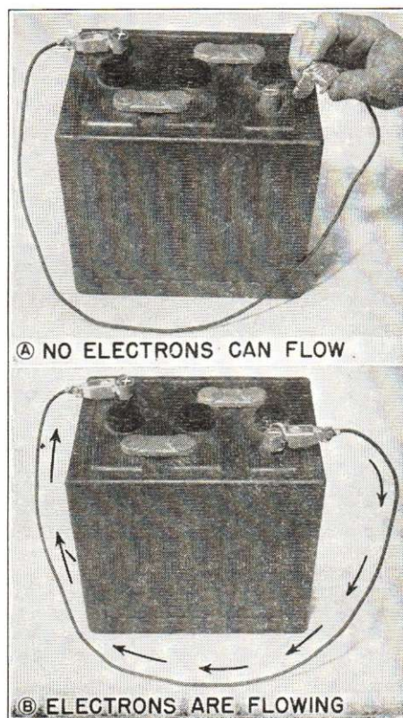
FIG. 3. Nothing happens when a wire is connected to only one terminal of a battery. There must be a complete path for electrons between the two battery terminals in order for electrons to flow. CAUTION: Never "short" a battery needlessly with a wire.
