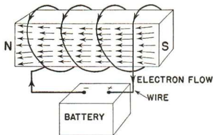
(B) IRON BAR MAGNETIZED BY CURRENT THROUGH COIL
