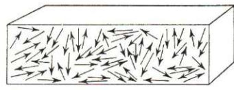
(A) UNMAGNETIZED IRON BAR
