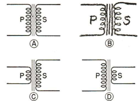
FIG. 21. Symbols for iron-core transformers.
