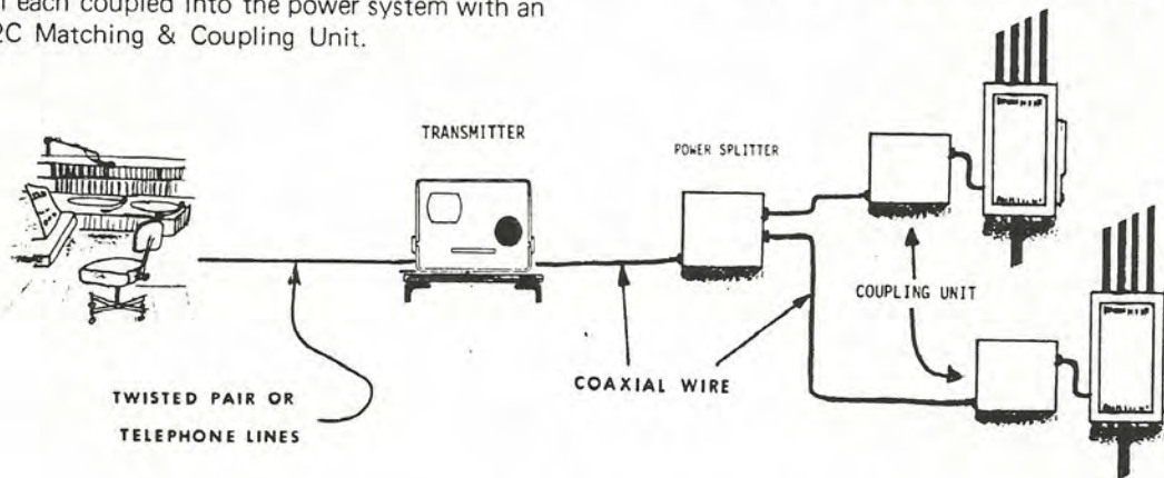
A Typical Installation, Showing Transmitter, 2-way Power Splitter and two Matching & Coupling Units
