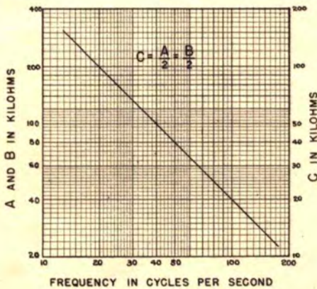
FIGURE 2. Resistor Values for Obtaining Other Frequencies
