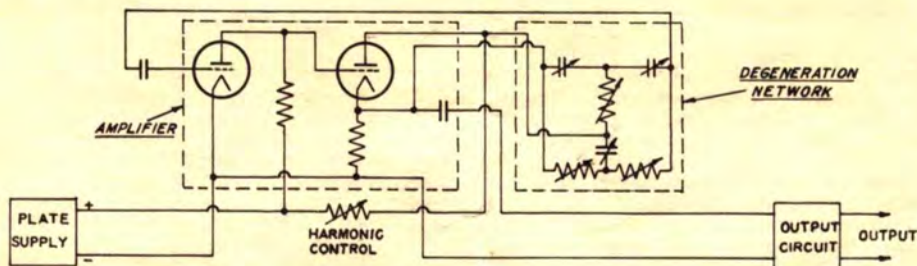
FIGURE 1. Functional Schematic Diagram of Type 608-A Oscillator
