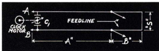
Fig. 4. Schematic diagram of the matching stub for use with untuned feedlines. The spacing "S" is about 1 inch. For 72-ohm twin lead, dimension "A" is about 18 inches, and "B" is about 6 inches. The over-all stub length is the same for other feedlines, but the tap position may change.
