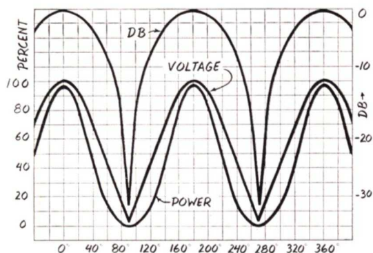
Fig. 3. Rectangular plot response pattern. The "DB" curve illustrates the same data as the polar plot, Fig. 1. Note that the "Power" curve is nearly a sine wave.
