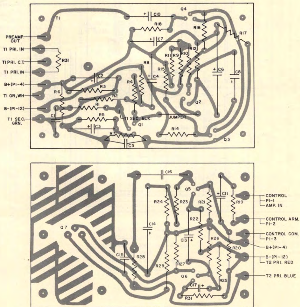
Fig. 6 - Printed Board Component Location, Viewed from Wiring Side.
