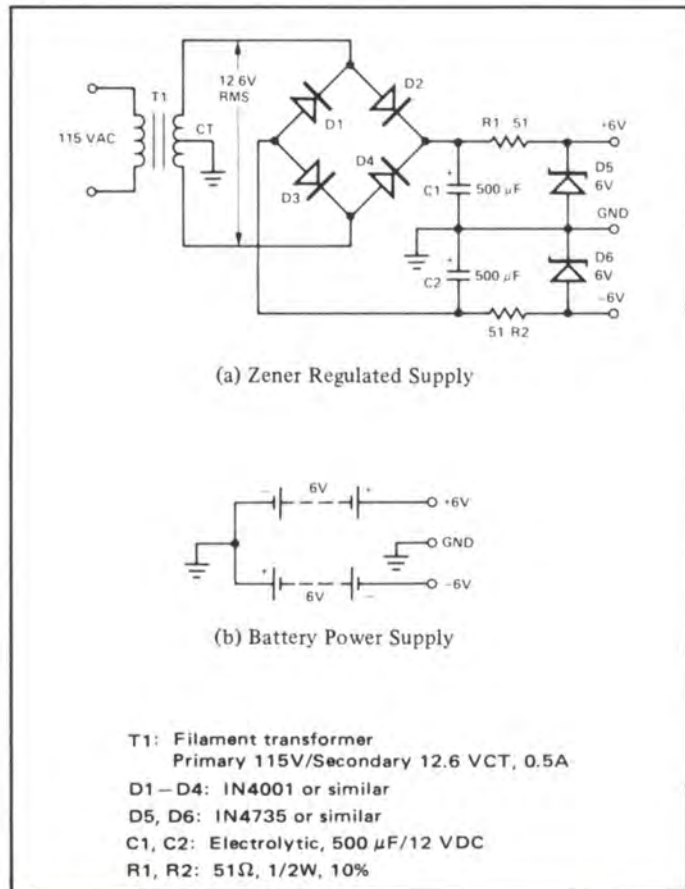
Figure 3. Recommended Power Supply Configurations.
