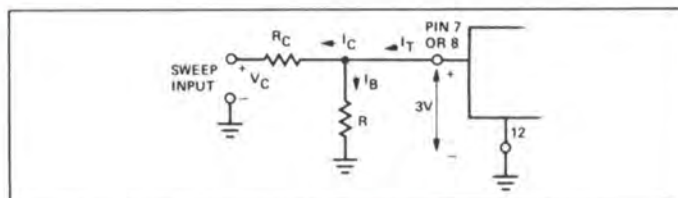
Figure 10. Circuit Connection for Frequency Sweep
