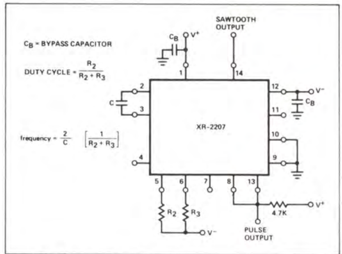
Figure 17. Sawtooth and Pulse Outputs
