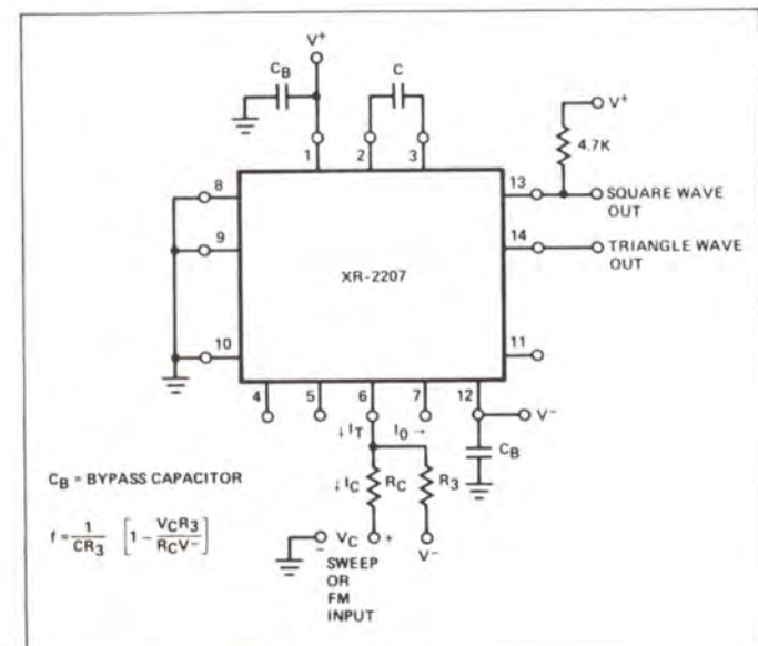
Figure 15. Frequency Sweep Operation
