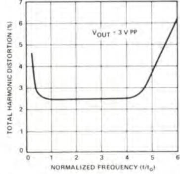
Figure 8. Sinusoidal Output Distortion as a Function of Frequency Sweep
