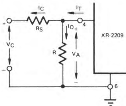
Figure 12. Frequency Sweep Operation
