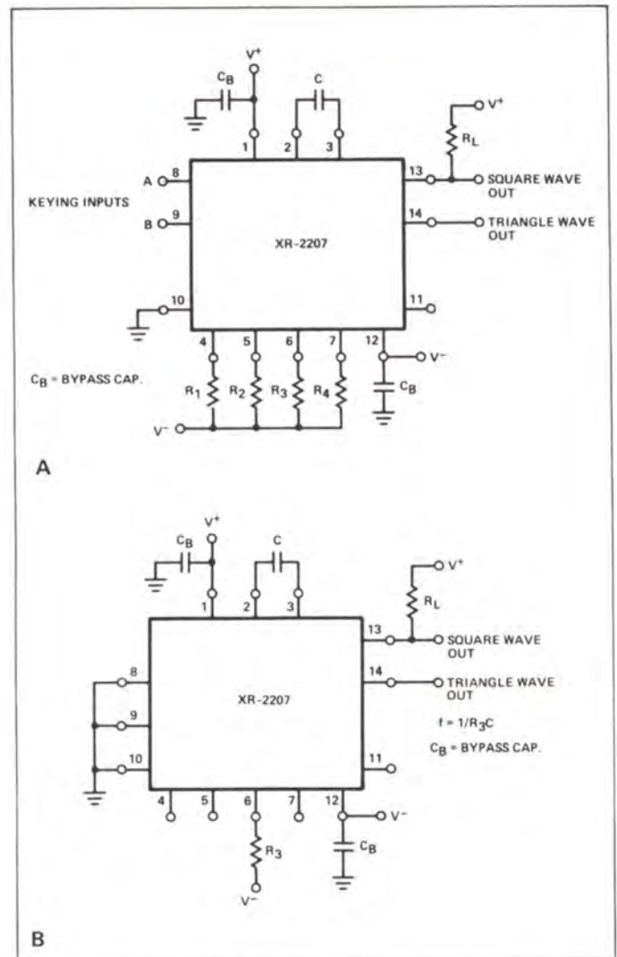
Figure 13. Split-Supply Operation:
