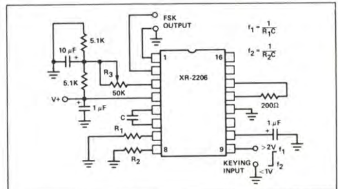
Figure 13. Sinusoidal FSK Generator
