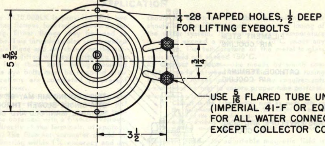
INPUT END VIEW
