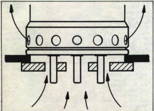
4-250A mounting providing base cooling, shielding and isolation of output and input compartments.
