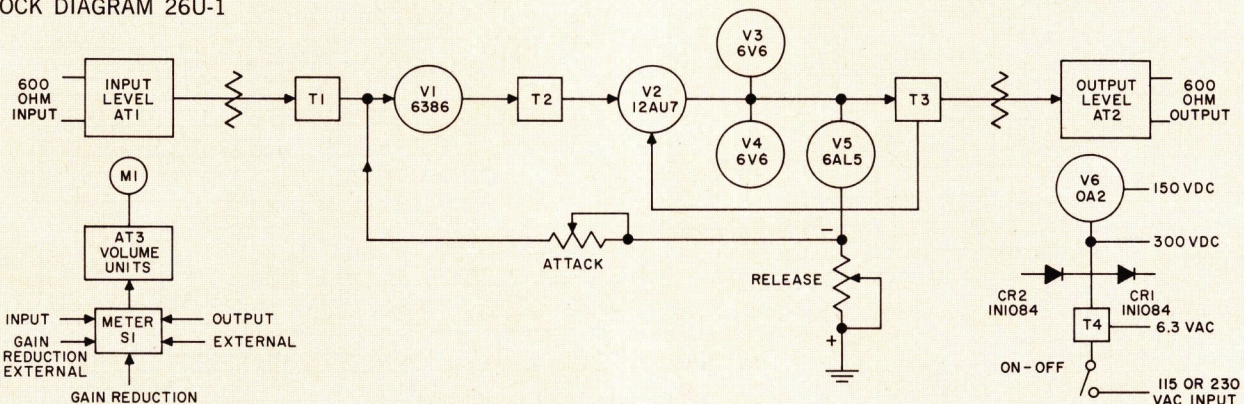
BLOCK DIAGRAM 26U-1
