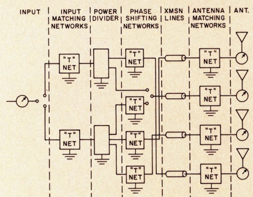
BLOCK DIAGRAM TYPICAL PHASING SYSTEM
