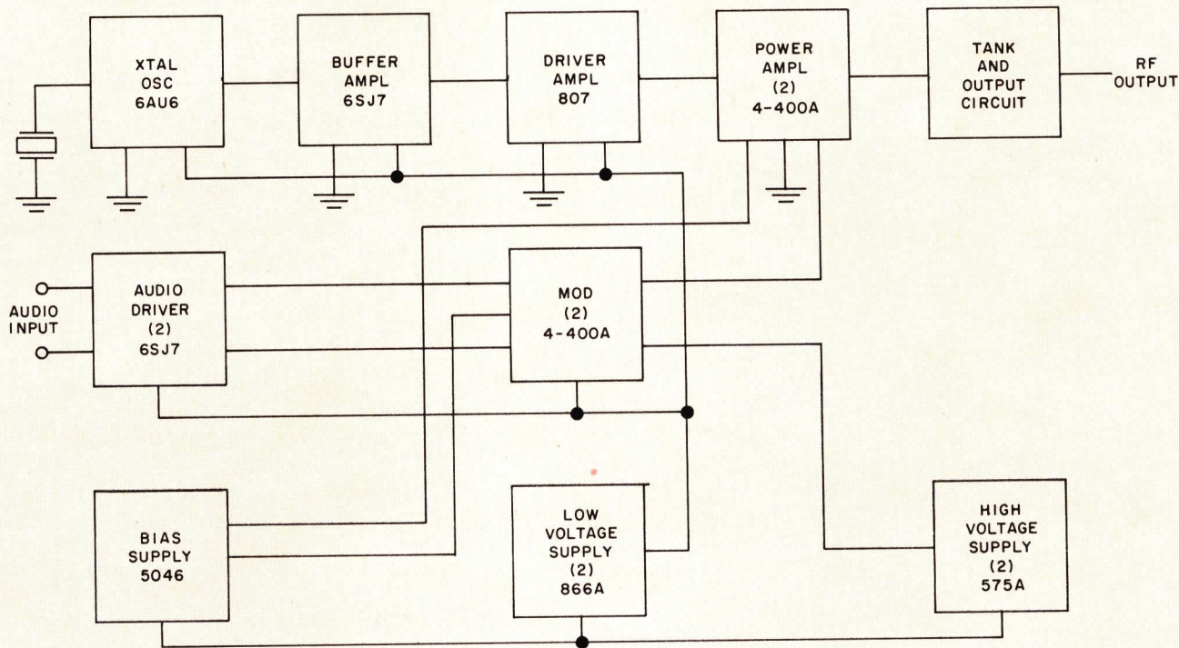
BLOCK DIAGRAM 20V-3
