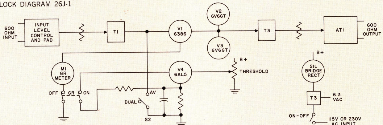
BLOCK DIAGRAM 26J-1
