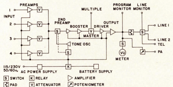
BLOCK DIAGRAM 212Z-1
