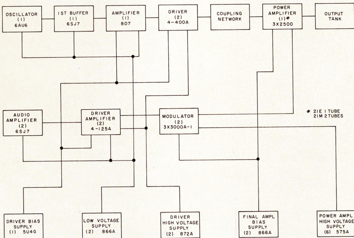
BLOCK DIAGRAM 21E/M
