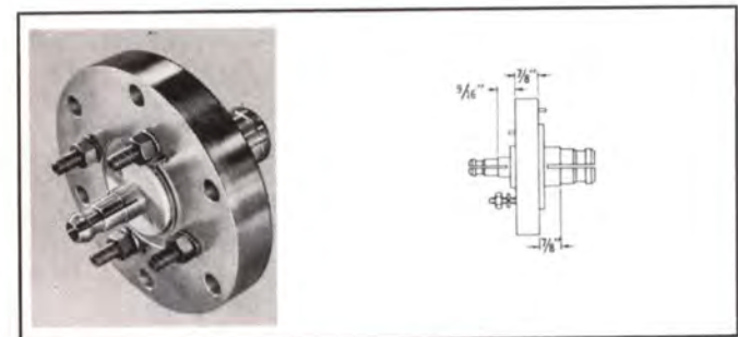
TYPE NO. 810-835 (NPN) — Reducer, flange type, 3 1/8" to 1 5/8" 50 ohm, incorporates 3 1/8" and 1 5/8" male anchor insulator connector. Includes 1 5/8" "O" ring, studs, nuts and lockwashers. Weight: 4 lbs. 13 oz.
