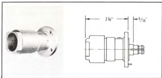
TYPE NO. 81-1025 (NPN) — Adapter assembly, 1 5/8" rigid to 1 5/8" EIA male, includes anchor insulator. Weight: 1 lb. 8 oz.
