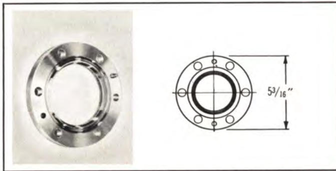
TYPE NO. 300-935 (NPN) — Flange, fixed, 6061 alloy. Weight: 8 \frac{1}{2} oz.
