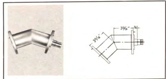
TYPE NO. 448-935 (NPN) — Elbow assembly, miter, 45 degree, swivel flanges. Includes one affixed male anchor insulator-connector, "O" ring and hardware. Weight: 3 \frac{1}{2} lbs.
