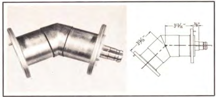
TYPE NO. 448-835 (Part No. 097 6633 00) — Elbow assembly, miter, 45 degree, female, reinforced, swivel flanged. Includes one anchor insulator-connector, "O" ring and hardware. Weight: 7 lbs.
