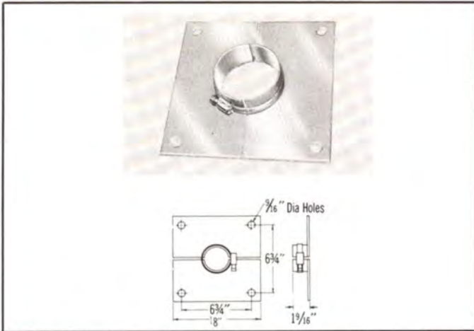
TYPE NO. 205-835 (NPN) — Anchor plate for anchoring single line at point of entry through a wall. One anchor required on each side of wall. Mounting bolts not supplied. Weight: 2 lbs. 12 oz.
