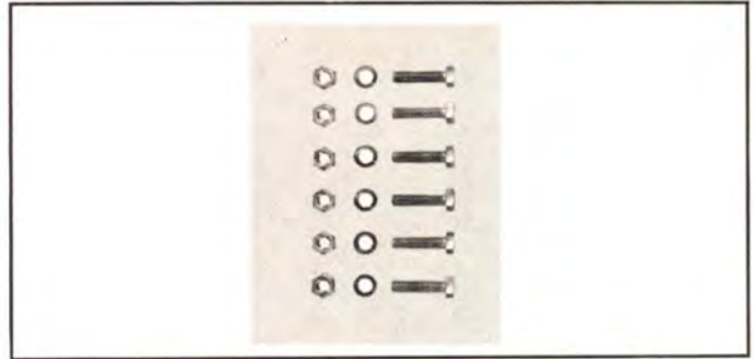
TYPE NO. 315-935 (NPN) — Hardware set, consists of 6 each stainless steel bolts, nuts and lockwashers, \frac{3}{8} "-16 x 1\frac{1}{2} " lg. Weight: 8 \frac{1}{2} oz.
