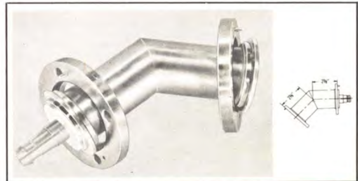
TYPE NO. 448-825 (Part No. 097 7511 00) — Elbow assembly, miter, 45 degree, female, swivel flanged. Includes one anchor insulator-connector, "O" ring and hardware. Weight: 2 lbs. 12 oz.
