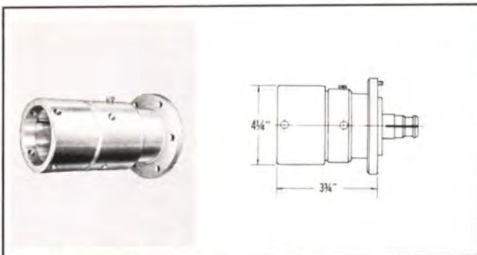
TYPE NO. 81-1035 (NPN) — Adapter Assembly, 3 1/8" rigid to 3 1/8" EIA, male, includes anchor insulator-connector. Weight: 3 lbs. 5 oz.
