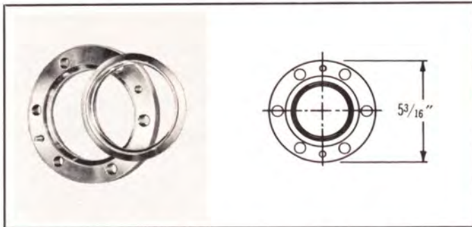
TYPE NO. 324-835 (NPN) — Flange, swivel, 5 3/16" dia., for silver brazing. Includes silver solder ring insert. Weight: 1 1/2 lbs.
