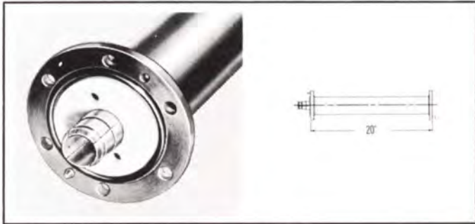
TYPE NO. 100-835 (Part No. 097 6631 —) — Line assembly, 20 ft. exact length flanged both ends. Includes anchor insulator-connector assembly, "O" ring and hardware. Weight: 54 1/2 lbs.
