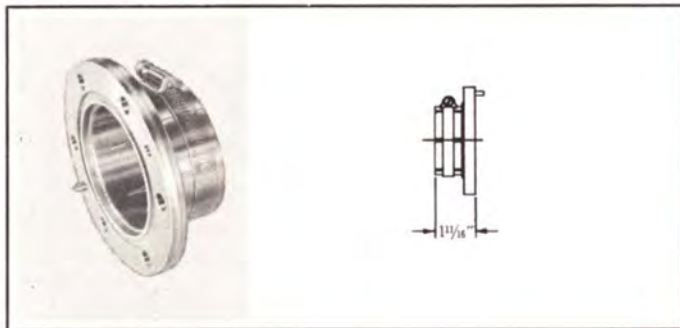
TYPE NO. 325-835 (NPN) — Adapter assembly, flanged to unflanged line, unpressurized, clamp type, for indoor use, includes hardware. Weight: 2 1/2 lbs.
