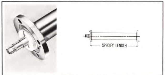
TYPE NO. 102-825 (NPN) — Line assembly, length to be specified, flanged both ends. Includes anchor-insulator connector assembly, "O" ring and hardware. Weight: 2 lbs. + 1 lb. 3 oz./ft.
