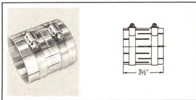
TYPE NO. 305-935 (NPN) — Coupling, straight, zinc plated, clamp type, unpressurized. Includes 2 tube clamps. No inner conductor-conector. Weight: 1 lb. 2 oz.
