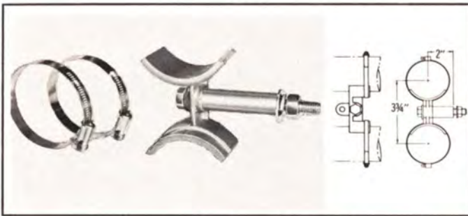
TYPE NO. 202-825 (NPN) — Hanger, fixed, direct attached, dual line. Mounts through \frac{1}{8} " dia. hole. Line clamps and hardware supplied. Weight: 1 lb. 6 oz.
