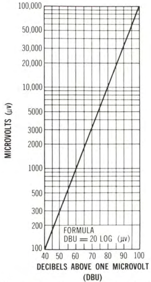
Transformation of microvolts to decibels above 1 \mu v .
