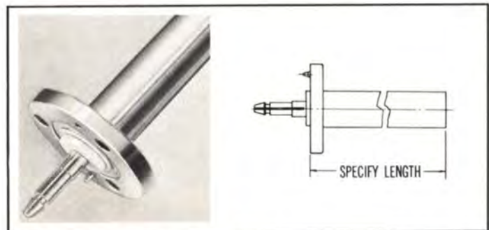
TYPE NO. 105-815 (NPN) — Line assembly, length to be specified, flanged one end. Includes anchor insulator connector assembly, "O" ring and hardware. Weight: 5 1/2 oz. + 5 1/2 oz./ft.
