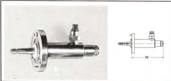
TYPE NO. 521-815 (NPN) — Adapter, EIA flange to type "N" female (UG-23D/U). Includes anchor insulator-connector, "O" ring and hardware. Incorporates 1/8" IPS port. Weight: 11 oz.
