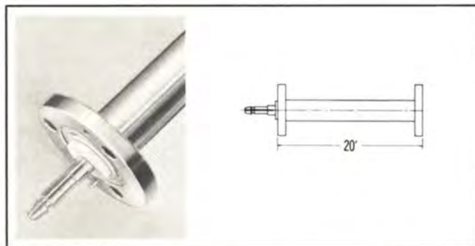
TYPE NO. 100-815 (NPN) — Line assembly, 20 ft. exact length, flanged both ends. Includes anchor insulator connector assembly, "O" ring and hardware. Weight: 11 lbs. 10 oz.
