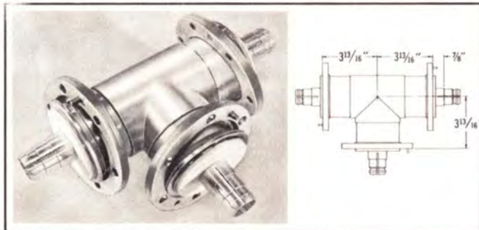
TYPE NO. 420-835 (NPN) — Tee assembly, reinforced, swivel flanges on all three legs, 3 13/16" center lines, affixed male anchor insulators all legs, includes "O" rings and hardware. Weight: 10 1/2 lbs.
