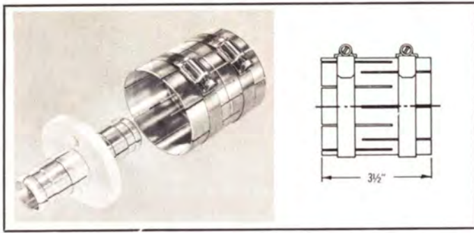
TYPE NO. 323-835 (NPN) — Coupling assembly, straight, clamp type, unpressurized. Includes inner conductor-connector assembly. (Special). Weight: 1 lb. 12 oz.
