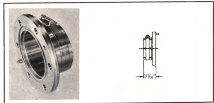
TYPE NO. 325-935 (NPN) — Adapter assembly, zinc plated, flanged to unflanged line, unpressurized, clamp type, for indoor use, includes hardware. Weight: 2 lbs. 8 oz.
