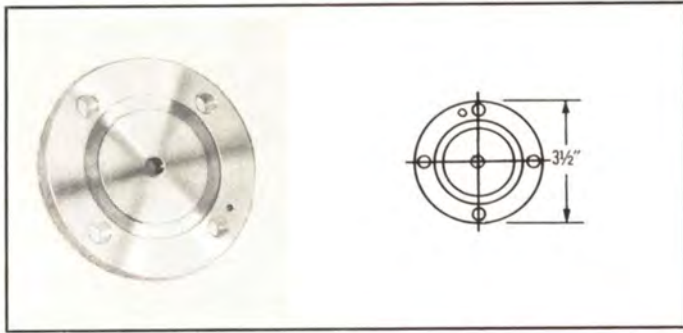
TYPE NO. 312-825 (NPN) — Cover plate, brass, with \frac{1}{8} " IPS gas inlet port and plug. No hardware. Weight: 1 lb.
