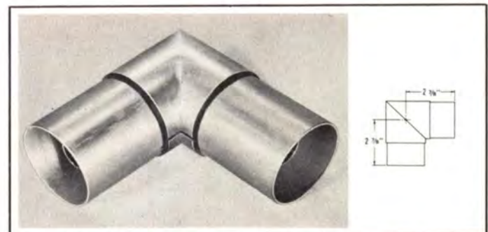
TYPE NO. 493-825 (NPN) — Elbow assembly, miter, 90 degree, female, reinforced, no flanges, equal legs. Inner conductor each leg cutback \frac{1}{8} " from face of outer conductor. Weight: 15 oz.
