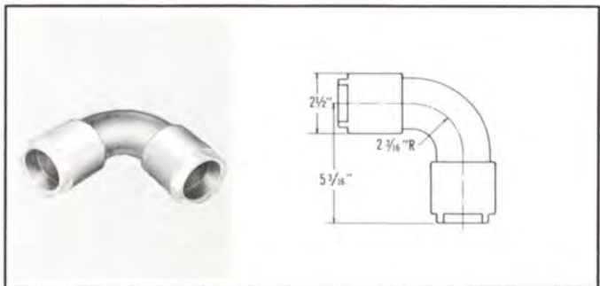
TYPE NO. 485-1025 (NPN) — Elbow assembly, sweep, 90° aluminum with Spir-O-lok connector. Weight: 3 1/2 lbs.
