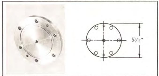
TYPE NO. 312-835 (NPN) — Cover plate, brass, with 1/8" IPS gas inlet port and plug. No hardware. Weight: 2 lbs. 3 oz.
