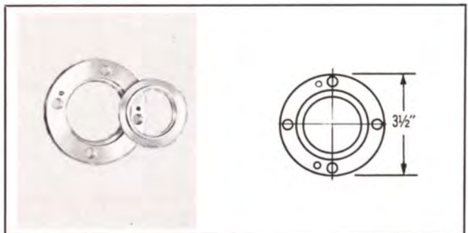
TYPE NO. 324-925 (NPN) — Flange, swivel, 6061 alloy. Weight: 4 1/2 oz.
