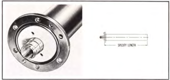
TYPE NO. 105-835 (NPN) — Line assembly, length to be specified, flanged one end. Includes anchor insulator-connector assembly, "O" ring and hardware. Weight: 3 lbs. + 2 1/2 lbs./ft.
