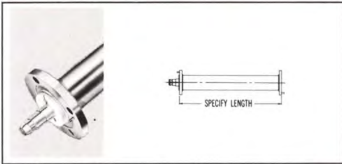
TYPE NO. 102-925 (NPN) — Line assembly, length to be specified, flanged both ends. Includes anchor insulator assembly, “O” ring and hardware. Weight: 1 lb. 3 oz. + 10 oz./ft.
