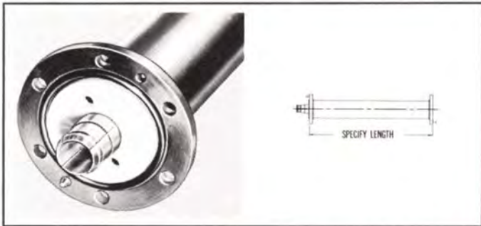
TYPE NO. 102-835 (NPN) — Line assembly, length to be specified, flanged both ends. Includes anchor insulator-connector assembly, "O" ring and hardware. Weight: 4 1/2 lbs + 2 1/2 lbs./ft.
