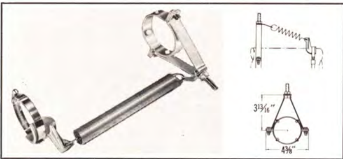
TYPE NO. 203-825 (NPN) — Hanger, spring suspension, direct attached, single line. Mounts through \frac{1}{8} " dia. hole. Line clamps and hardware supplied. Weight: 2 \frac{1}{2} lbs.
