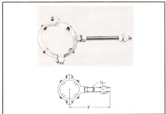
TYPE NO. 212-835 (NPN) — Hanger, slip type, 7" stud mount (1/2"-13 thread). Weight: 1 lb. 12 oz.
