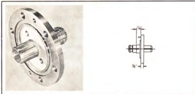
TYPE NO. 304-835 (NPN) — Adapter, flange type, includes anchor insulator-connector. Used for connecting flanged, 50 ohm EIA line to flanged 51.5 ohm RMS-VHF line with inner conductor 1.200 O.D. x 1.136 I.D. Supplied with "O" ring and hardware. Weight: 2 lbs. 9 oz.
