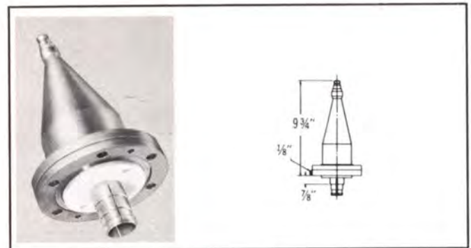
TYPE NO. 521-835 (NPN) — Taper, 3 1/8" — 50 ohm to Type "N" female. Includes anchor insulator assembly, "O" ring, nuts and lockwashers. Weight: 7 1/2 lbs.
