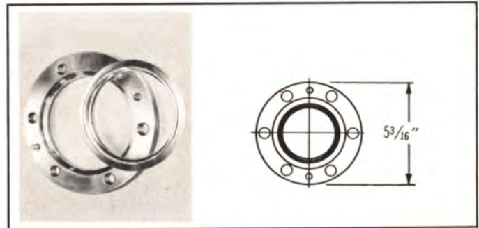
TYPE NO. 324-935 (NPN) — Flange, swivel, 6061 alloy. Weight: 8 \frac{1}{2} oz.
