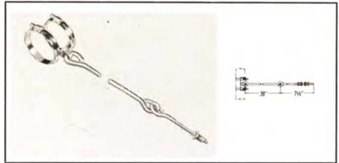
TYPE NO. 208-825 (NPN) — Lateral brace for securing transmission line at base of tower. Complete with clamps. Weight: 2 lbs. 5 oz.
