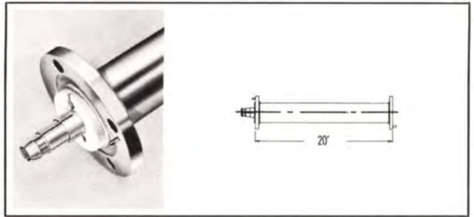
TYPE NO. 100-825 (Part No. 097 7081 —) — Line assembly, 20 ft. exact length, flanged both ends. Includes anchor insulator-connector assembly, "O" ring and hardware. Weight: 26 lbs.
