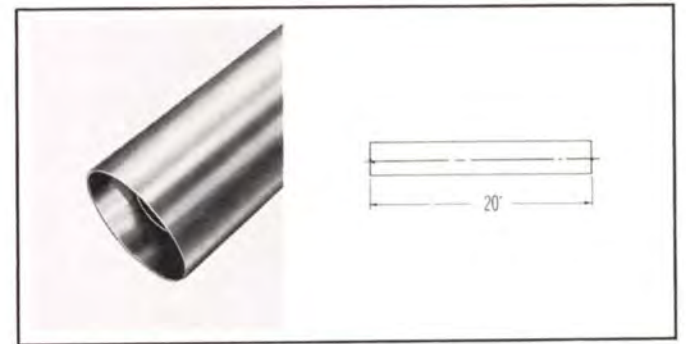
TYPE NO. 101-925 (NPN) — Coaxial line assembly, 20 ft. exact length, no flange. Weight: 12 1/2 lbs.
