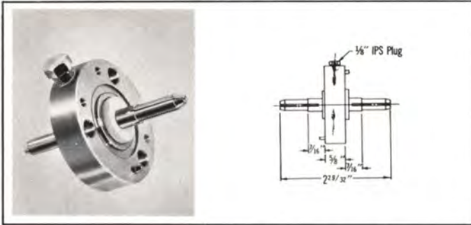
Type No. 500-815 (NPN) — Gas barrier, with "O" ring and extra long hardware. Incorporates 1/8" IPS gas inlet port. Weight: 13 oz.
