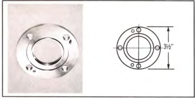
TYPE NO. 300-925 (NPN) — Flange, fixed, 6061 alloy. Weight: 4 1/2 oz.
