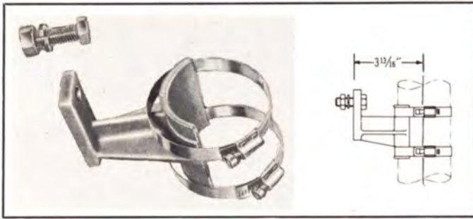
TYPE NO. 201-825 (NPN) — Hanger, fixed, direct attached, single line. Mounts through \frac{1}{8} " dia. hole. Line clamp and hardware supplied. Weight: 1 lb. 4 oz.
