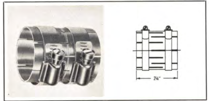
TYPE NO. 305-825 (NPN) — Coupling, straight clamp type, unpressurized. Includes 2 tube clamps. No inner conductor connector. Weight: 5 1/2 oz.
