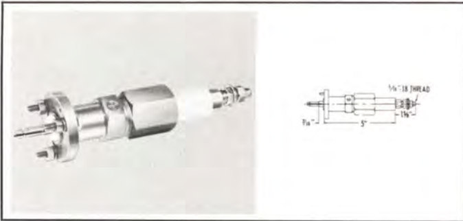
TYPE NO. 505-815 (NPN) — End seal assembly, flanged with gas inlet port, includes "O" ring and hardware. Weight: 1 lb.
