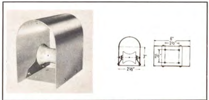
TYPE NO. 209-825 (NPN) — Roller assembly consisting of roller, bracket and hood for outdoor horizontal transmission line runs. Weight: 1 lb. 5 oz.
