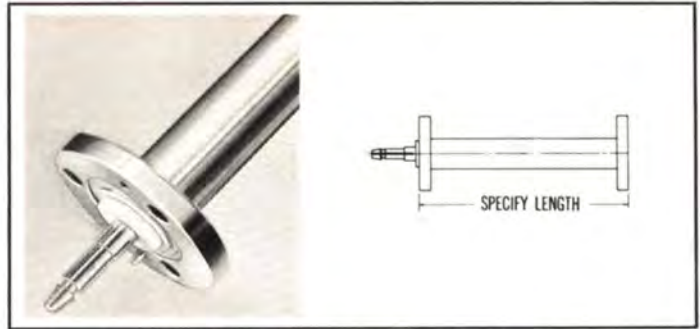
TYPE NO. 102-815 (NPN) — Line assembly, length to be specified, flanged both ends. Includes anchor insulator connector assembly, "O" ring and hardware. Weight: 10 oz. + 5 1/2 oz./ft.
