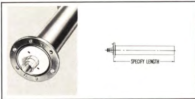
TYPE NO. 105-935 (NPN) — Line assembly, length to be specified, flanged one end. Includes anchor insulator-connector assembly, "O" ring and hardware. Weight: 2 lbs. + 1 lb. 5 oz./ft.
