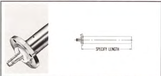
TYPE NO. 105-925 (NPN) — Line assembly, length to be specified, flanged one end. Includes anchor insulator-connector assembly, “O” ring and hardware. Weight: 12 oz. + 10 oz./ft.
