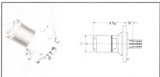
TYPE NO. 82-1025 (NPN) — Adapter assembly, 1 5/8" to 3 1/8" EIA male, includes anchor insulator-connector. Weight: 2 lbs. 6 oz.
