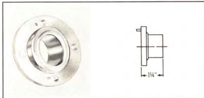
TYPE NO. 322-825 (NPN) — Adapter assembly, flange, swivel to unflanged line, soft solder type, pressurized. No anchor insulator-connector, "O" ring or hardware. Weight: 14 oz.
