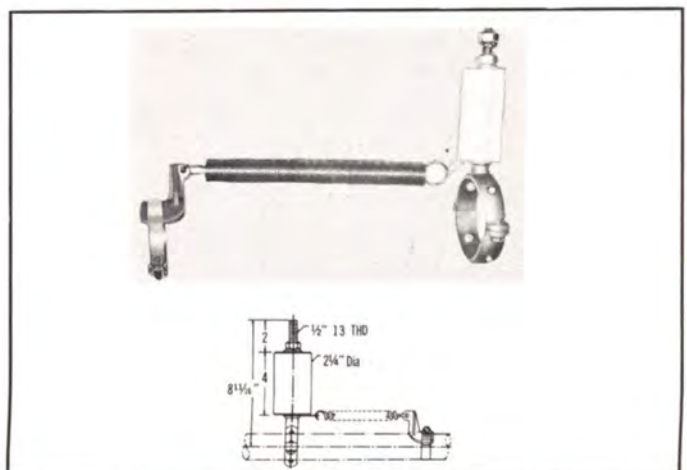
TYPE NO. 213-835 (NPN) — Hanger, insulated, direct attached. Mounts through 1/8" dia. hole. Hardware supplied. Weight: 5 lbs.
