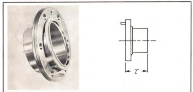
TYPE NO. 322-835 (NPN) — Adapter assembly, flanged to unflanged line, soft solder type, pressurized. No anchor insulator-connector, "O" ring or hardware. Weight: 2 lbs.
