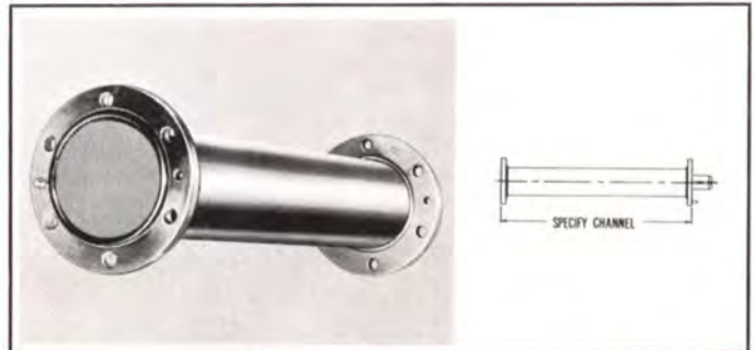
TYPE NO. 130-835 (NPN) — Transformer, 1/4 wave, used to join 50 ohm line to 51.5 ohm RMA line. Specify channel from 2 to 13. Connector for 51.5 ohm end supplied. Weight varies with channel.
