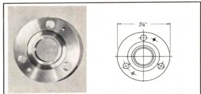
TYPE NO. 300-815 (NPN) — Flange, fixed, for silver brazing. Includes silver solder ring insert. Weight: 4 oz.
