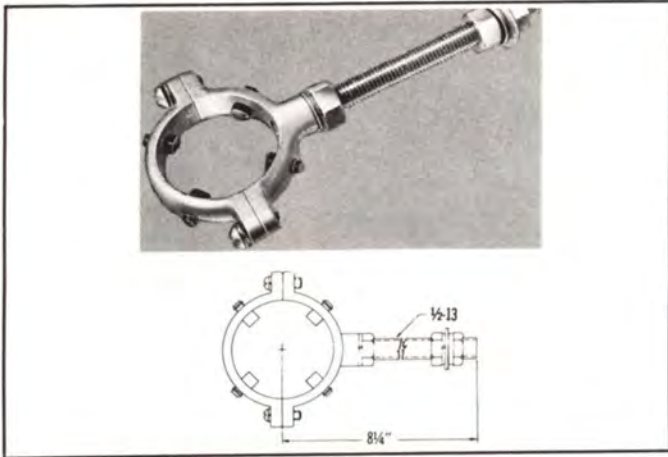
TYPE NO. 212-825 (NPN) — Hanger, slip type, 7" stud mount ( \frac{1}{2} "-13 thread. Weight: 1 lb. 3 oz.
