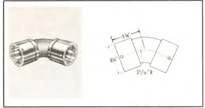
TYPE NO. 490-1035 (NPN) — Elbow assembly, sweep, 45° cast aluminum with Spir-O-lok connectors, both male ends. Weight: 5 lbs. 3 1/2 oz.
