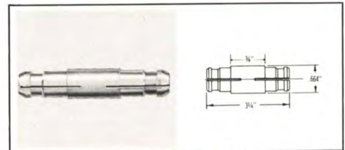
TYPE NO. 310-825 (Part No. 099 0459 00) — Inner conductor connector, silver plated. Weight: 2 1/2 oz.
