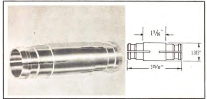
TYPE NO. 310-835 (Part No. 097 6635 00) — Inner conductor connector only, silver plated, spring loaded. Used with Type No. 305-835. Weight: 7 oz.
