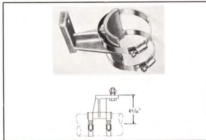
TYPE NO. 201-835 (NPN) — Hanger, fixed, direct attached, single line. Mounts through \frac{1}{8} " dia. hole. Line clamp and hardware supplied. Weight: 2 lbs. 4 oz.
