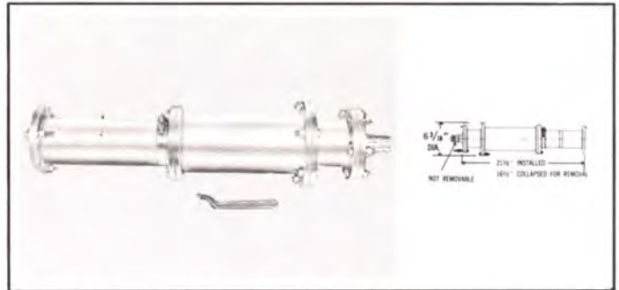
TYPE NO. 120-835 (NPN) — Breakaway section, EIA flanged both ends, permits separating the transmission line at any convenient point. Pressure tight. Weight: 14 lbs.
