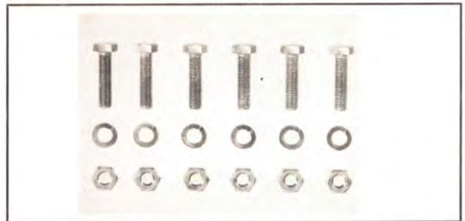
TYPE NO. 315-835 (NPN) — Hardware set for 3 1/8" flanges. Consists of 6 ea. stainless steel bolts, nuts and lockwashers, 3/8"-16 x 1 1/2" lg. Weight: 8 1/2 oz.
