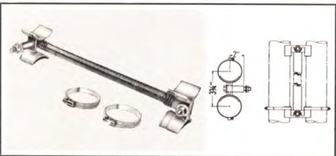
TYPE NO. 204-825 (NPN) — Hanger, spring suspension, direct attached, dual line. Mounts through \frac{1}{8} " dia. hole. Line clamps and hardware supplied. Weight: 3 lbs.
