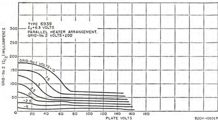
AVERAGE GRID-No. 2 CHARACTERISTICS EACH UNIT
