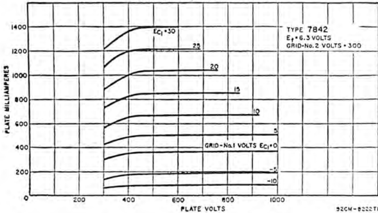
TYPICAL PLATE CHARACTERISTICS
