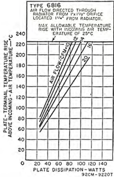
TYPICAL COOLING REQUIREMENTS
