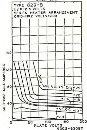
TYPICAL CHARACTERISTICS EACH UNIT
