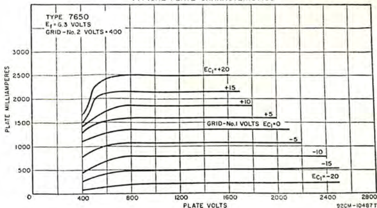
TYPICAL PLATE CHARACTERISTICS
