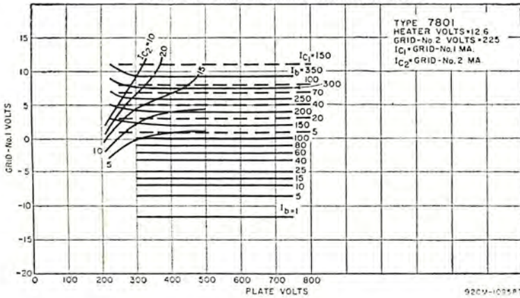
TYPICAL CONSTANT-CURRENT CHARACTERISTICS
