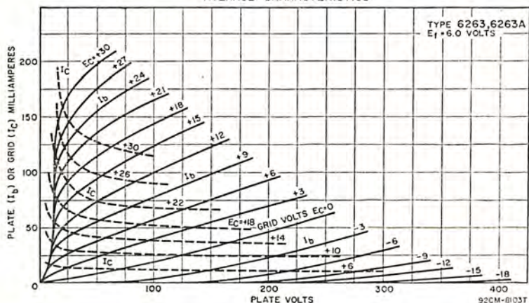
AVERAGE CHARACTERISTICS
