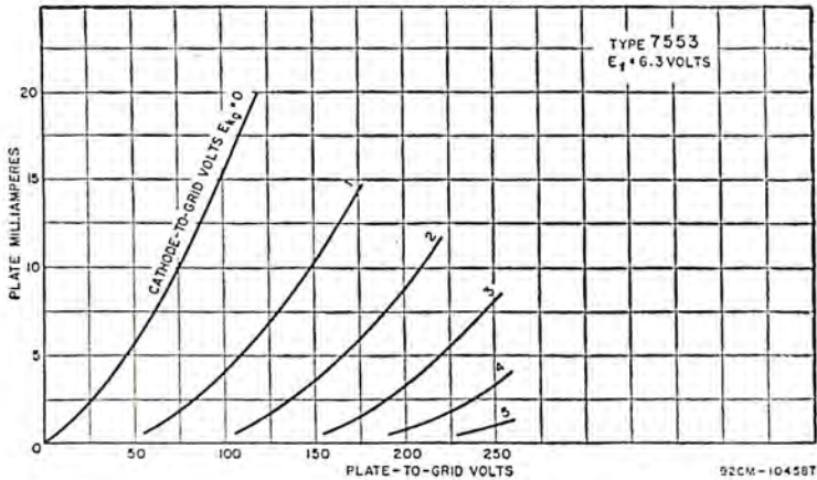
GAIN CHARACTERISTICS CATHODE - DRIVE SERVICE
