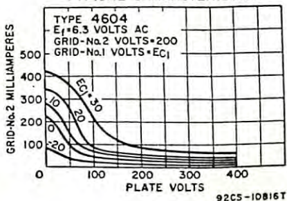
TYPICAL CHARACTERISTICS
