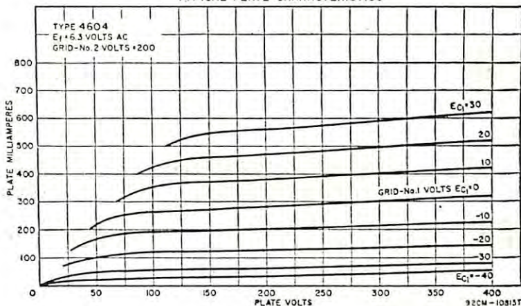
TYPICAL PLATE CHARACTERISTICS
