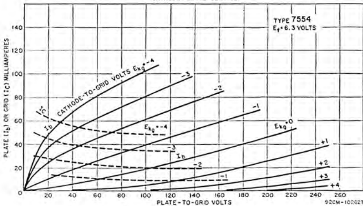
AVERAGE CHARACTERISTICS CATHODE-DRIVE SERVICE
