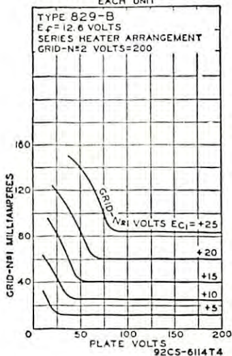
TYPICAL CHARACTERISTICS EACH UNIT
